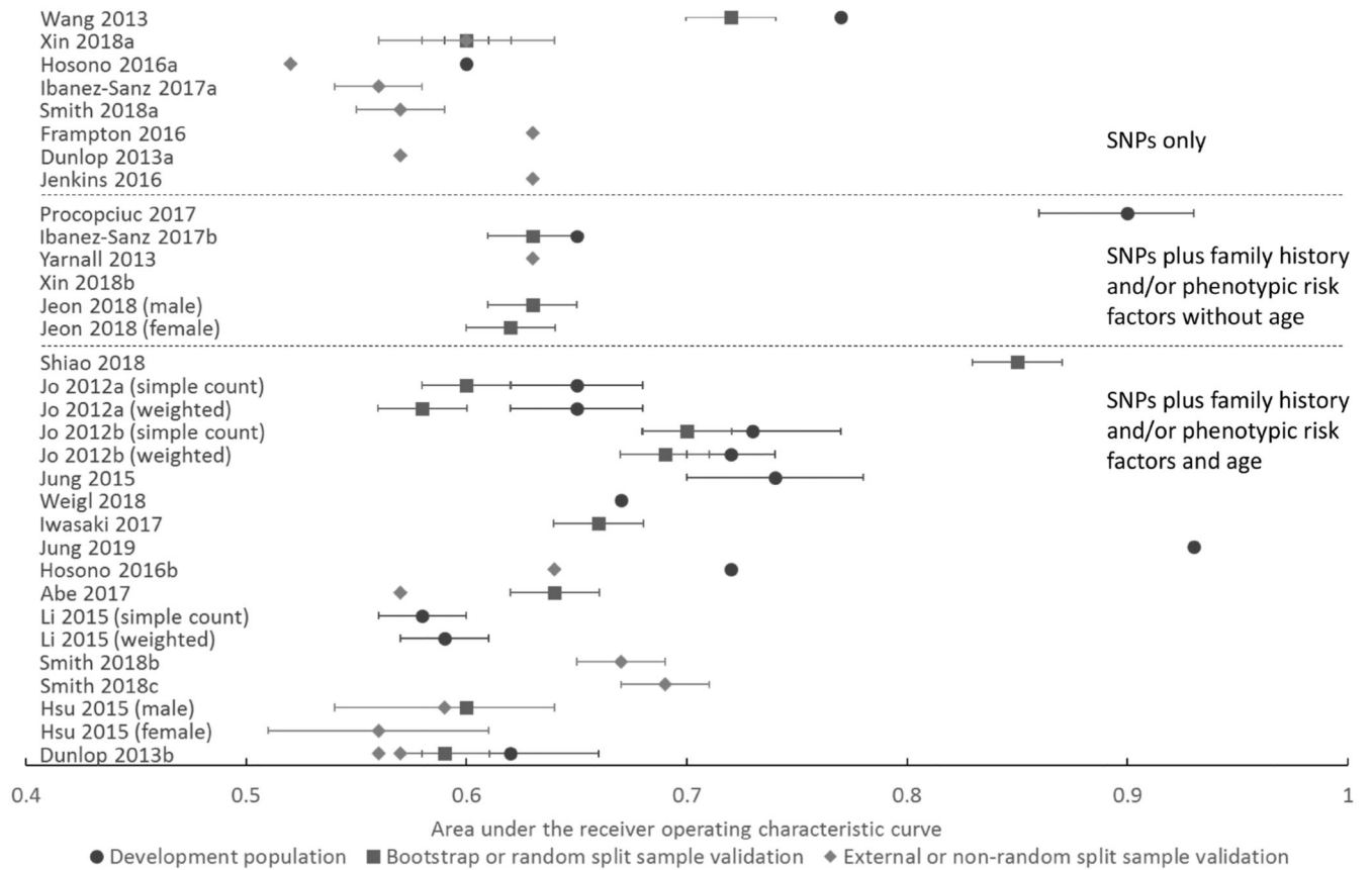
Figure 1. Relative discriminative performance of the risk scores grouped by those including only SNPs, those including SNPs plus family history and/or phenotypic risk factors without age and those including SNPs plus family history and/or phenotypic risk factors and age. Within each of these groups, the models are ordered according to sample size, with larger studies being those towards the bottom of each risk model category.
