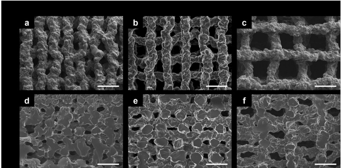
Figure 1. SEM images of 3-D printed silica-PTHF/PCL hybrid scaffolds with different vertical channel widths: a, d) images of SC-100 (mean channel width 117 \pm 42 \mu\text{m} ), printed with 0.5 mm strut spacing; b, e) images of SC-250 (mean channel width 231 \pm 54 \mu\text{m} ), printed with 0.6 mm strut spacing; c, f) images of SC-500 (mean channel width 503 \pm 82 \mu\text{m} ), printed with 1.0 mm strut spacing. a-b-c (top) shows images of the top surface; d-e-f (bottom) shows images of a vertical (z-y) section. Scale bars = 500 \mu\text{m} .
