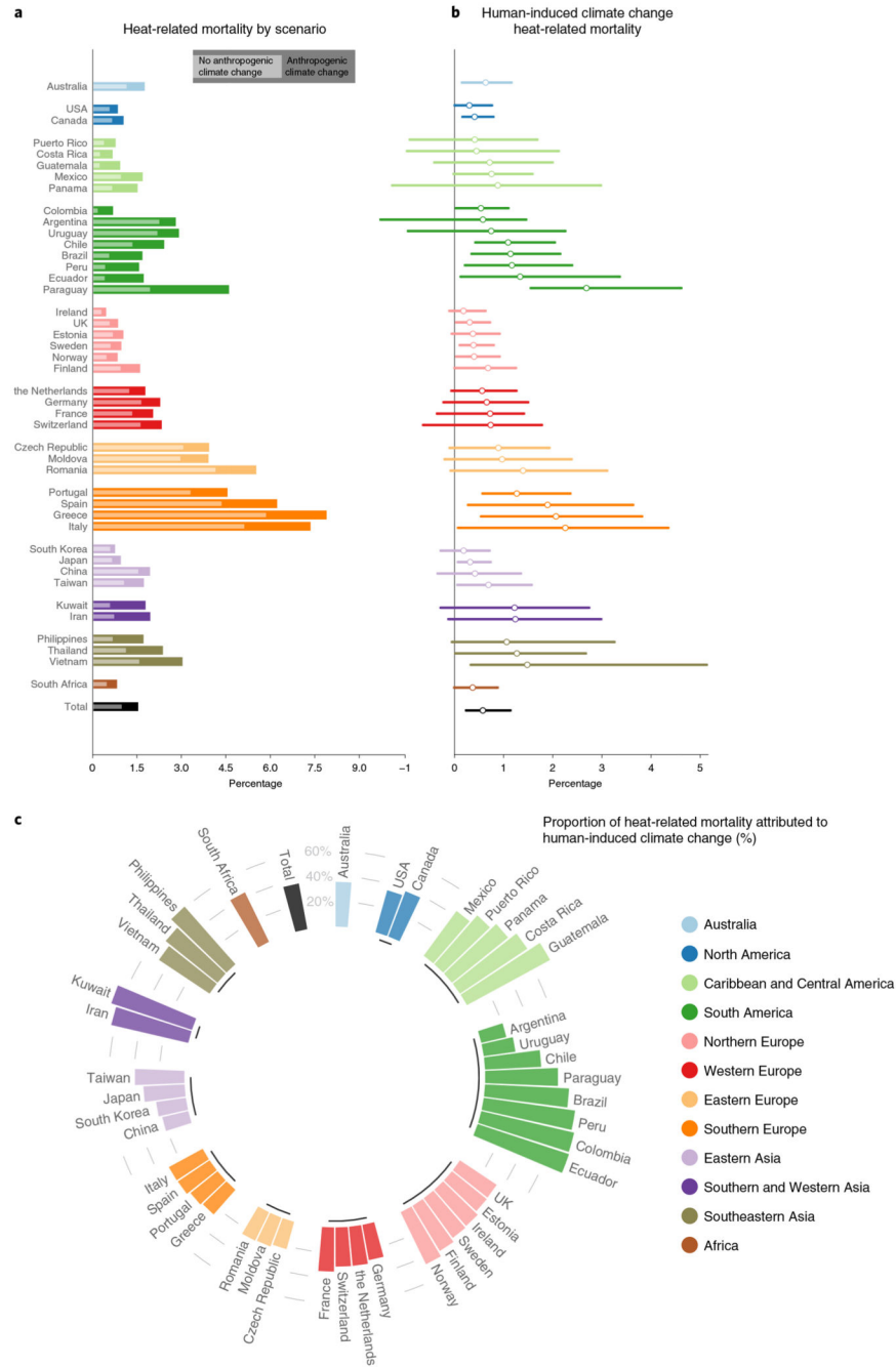
Fig. 4. Heat-related mortality and the contribution of human-induced climate change, 1991–2018.
