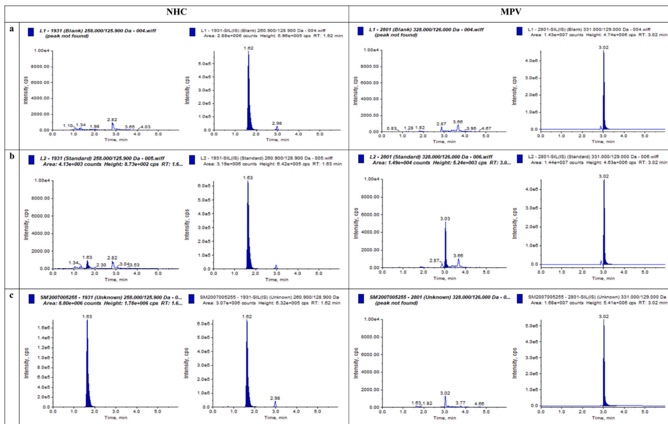
Fig. 1. Chromatograms of NHC and MPV in Plasma in (a) Blank extracted plasma sample; (b) Spiked with 2.5 ng/ml (LLOQ); (c) Patient sample, 4245.7 ng/ml NHC; MPV < LLOQ; all with internal standards.
