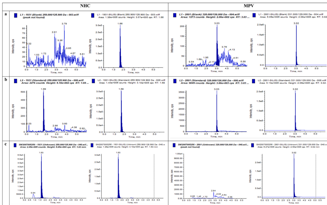
Fig. 2. Chromatograms of NHC and MPV in Saliva in (a) Chromatogram of Blank PBS sample; (b) Spiked with 2.5 ng/ml (LLOQ); (c) Patient sample, 230.0 ng/ml NHC ; MPV < LLOQ; all with internal standards.
