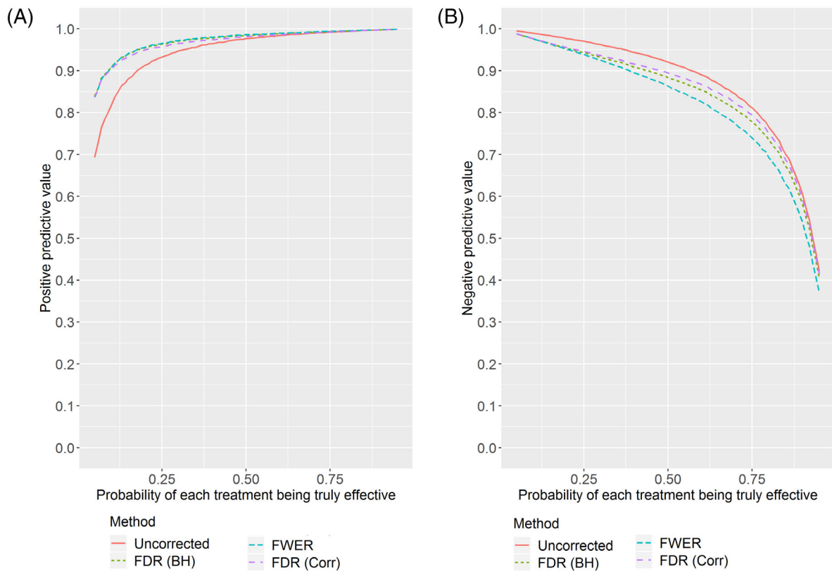
FIGURE 2 Positive and negative predictive values estimated from the simulation study with five experimental arms as the proportion of treatments which are truly effective changes. A, Positive predictive value. B, Negative predictive value
