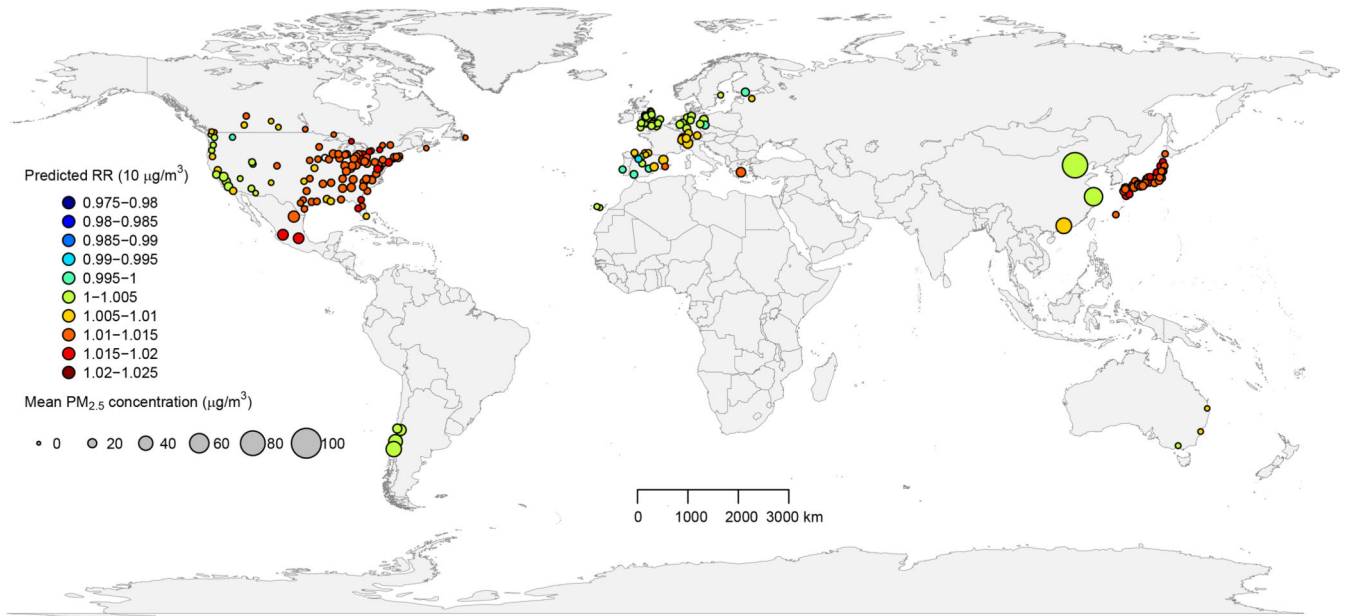
Figure 1. Locations used in the study with their mean PM 2.5 concentration and best linear unbiased predictions (BLUPs) of relative risks (RRs) per 10 µg/m 3 increase in PM 2.5 .
