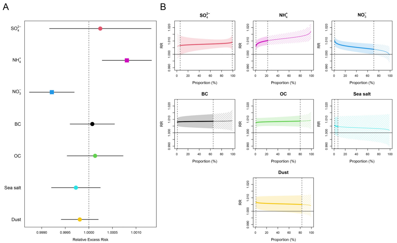
Figure 3. Effect modification from each PM 2.5 component. A: relative excess risk (RER) associated to doubling the relative proportion of each component with 95% confidence interval. B: predicted relative risks (RRs) for different values of each component while keeping the other constituents constant. The predicted RR is associated with an increase of 10µg/m 3 in PM 2.5 . Thick lines indicate the range of observed values for each component, while thin dashed lines indicate extrapolations. Colored bands represent 95% confidence regions.
