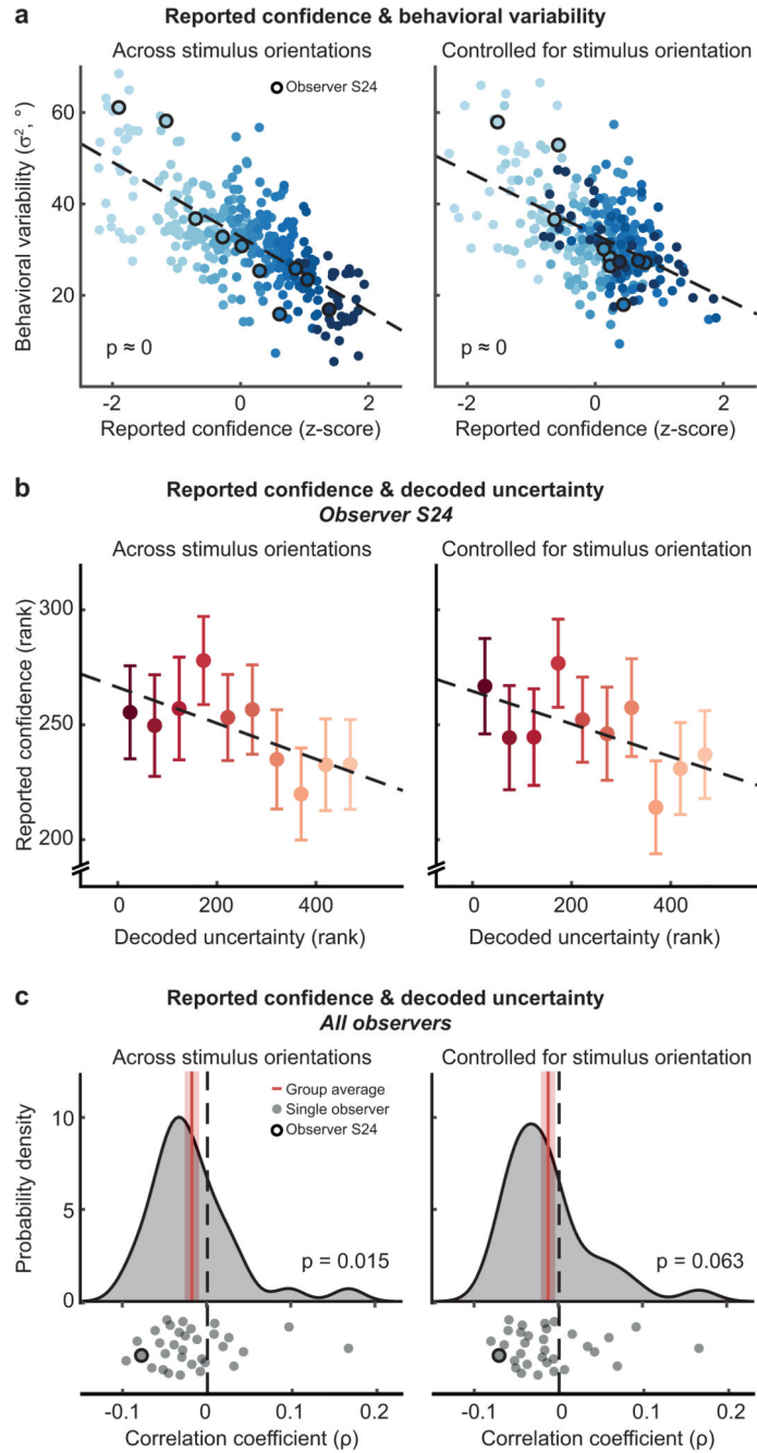
Fig. 3. Reported confidence, behavioral variability, and decoded sensory uncertainty.
