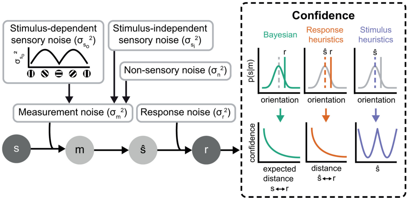
Fig. 1. Overview of sources of noise and three observer models.
