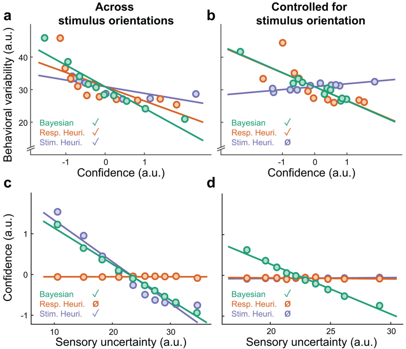
Fig. 2. Ideal observer predictions.
