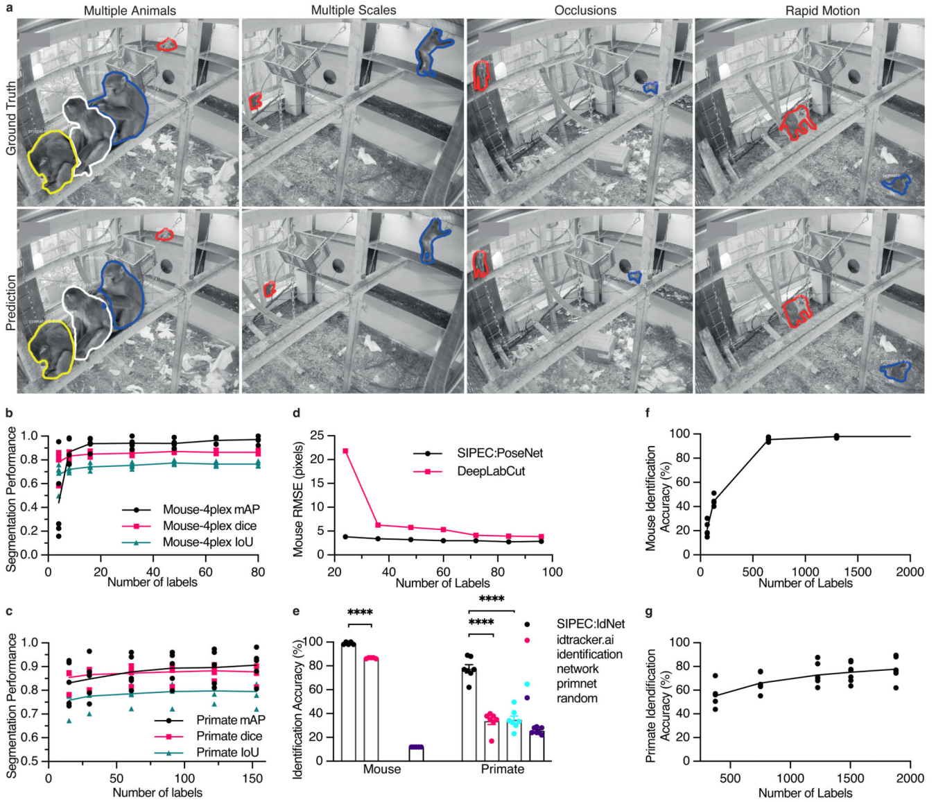
Fig. 2. Performance of the segmentation (SIPEC:SegNet), pose estimation (SIPEC:PoseNet), and identification (SIPEC:IdNet) modules under demanding video conditions and using few labels.
