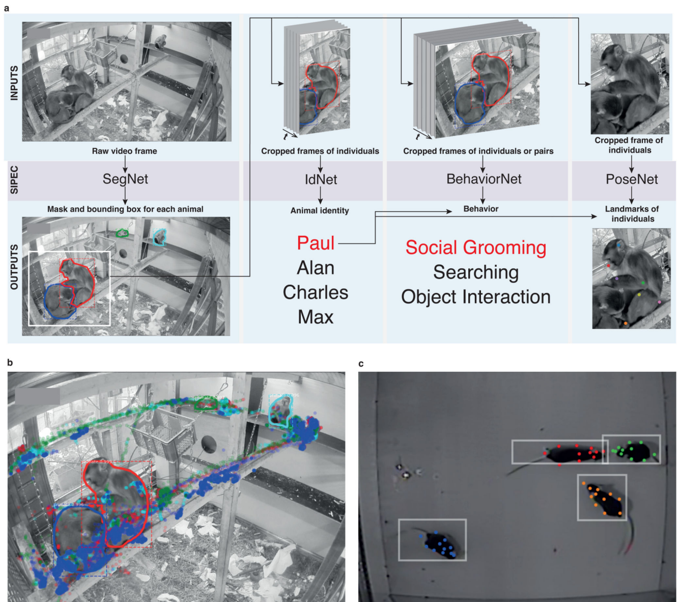
Fig. 1. Overview of the SIPEC workflow and modules.
