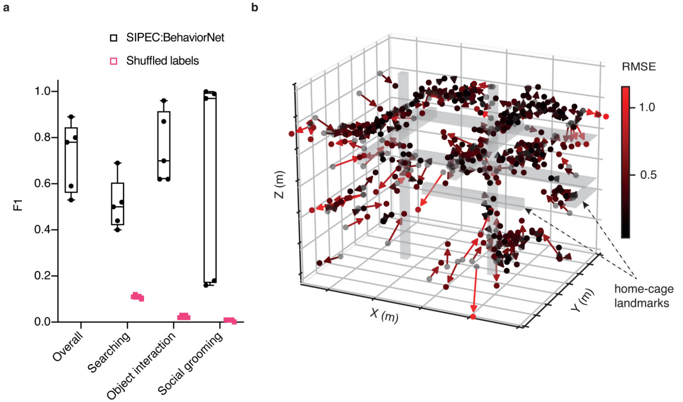
Fig. 4. SIPEC can recognize social interactions of multiple primates and infer their 3D positions using a single camera.
