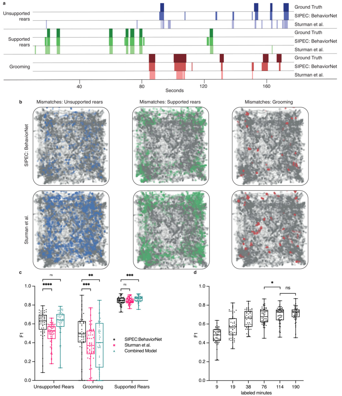
Fig. 3. SIPEC:BehaveNet outperforms pose-estimation (DeepLabCut) based approach (Sturman et al. 20 ).
