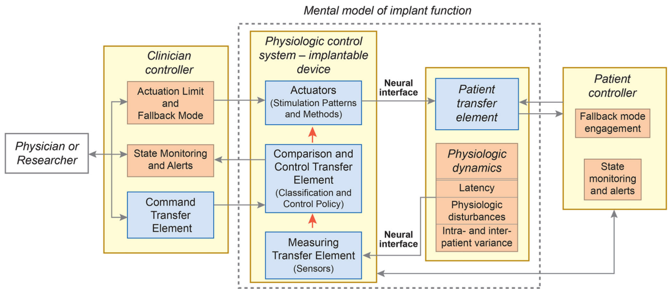
Fig. 1. System block-diagram using the IEC 60601-1-10 physiologic control framework [1]. Blue boxes are derived from user needs, while tan boxes are derived from risk mitigations. Both sources of design inputs inform the system specifications for the DyNeuMo Mk-1.
