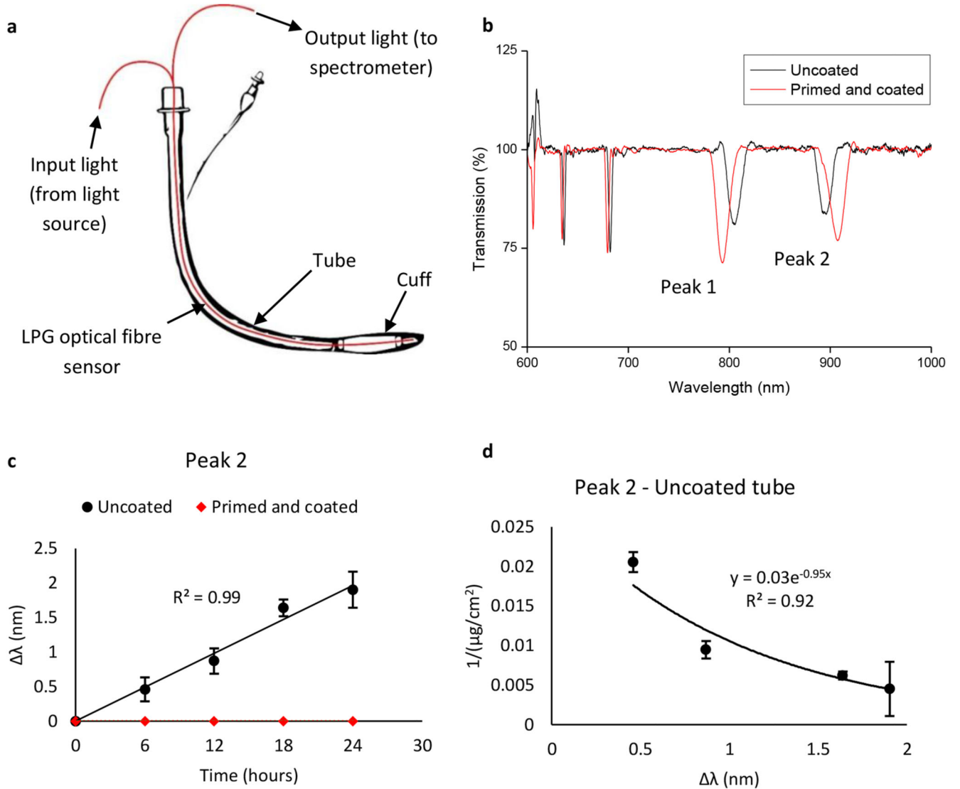
Figure 4. Response from LPG sensor instrumented ETT.
