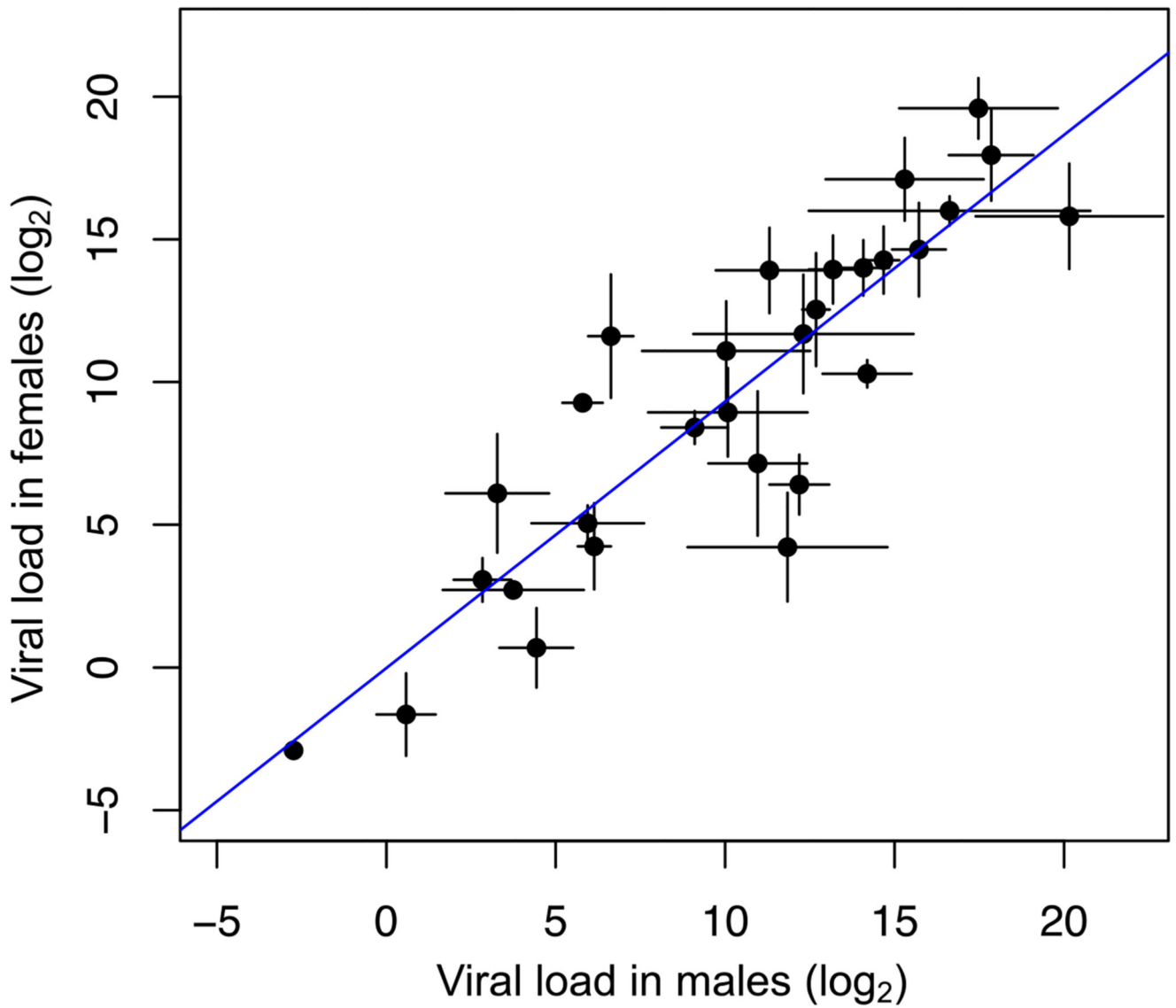
Figure 1. Correlation between viral load in males and females.
