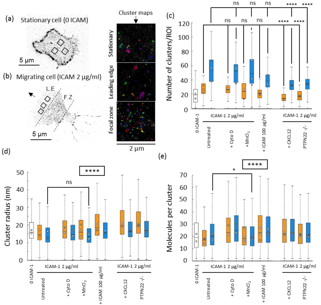
Figure 2. Integrin LFA-1 membrane nanoclusters increase in density and decrease in number in fast migrating cells.
