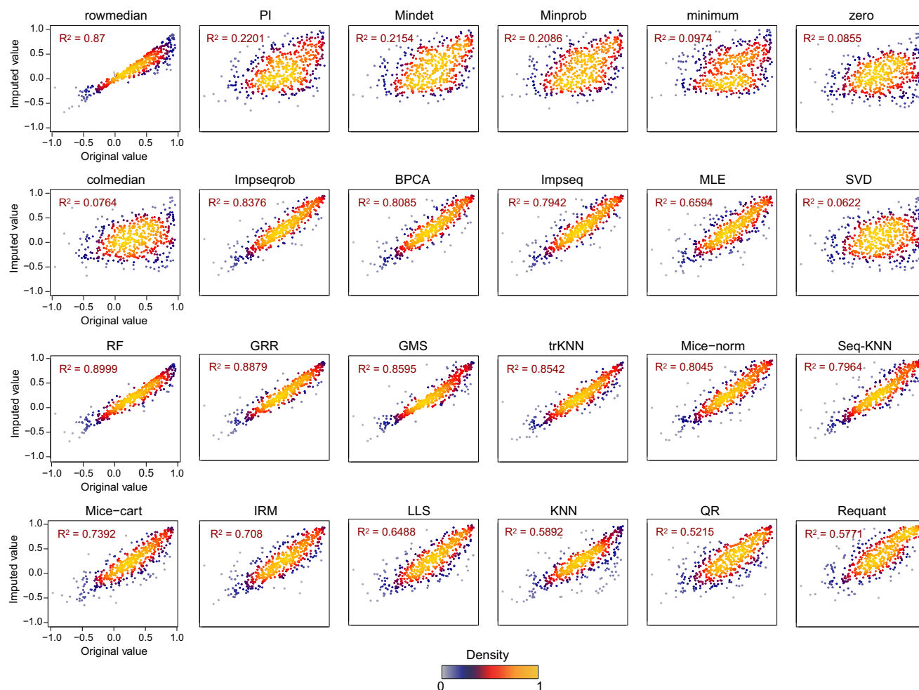
Figure 4. Across sample, quantitative correlation coefficients obtained by different NA imputation methods. Comparisons of original values and imputed values of the quantitative correlation coefficients are shown which are derived under ACC_Charge criterion by the 23 imputation methods and ‘Requantification’ method for the pepSWATH dataset. The adjusted R^2 of each result was also obtained by ‘lm’ function and shown for every imputation method. ‘Requant’ denotes ‘Requantification’ method in OpenSWATH software.
