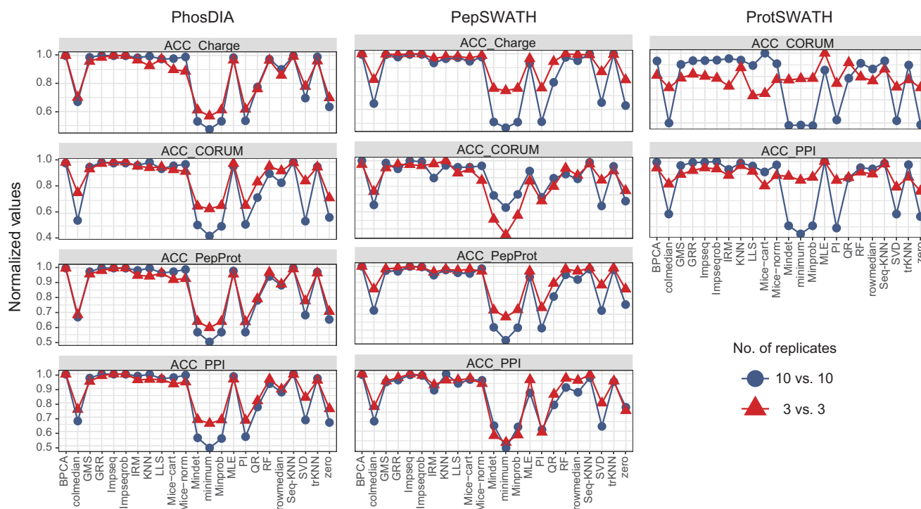
Figure 3. The score distribution of every imputation method based on the proteomic criteria in the three proteomics datasets with different biological replicates. Left panel: PhosDIA, middle: PepSWATH, right: ProtSWATH. ‘Normalized values’ denotes that every score is divided by corresponding maximum value. ‘10 versus 10’ means that there are 10 replicates in each group (marked with darkblue color), and ‘3 versus 3’ means that there are three replicates in each group (marked with red color).
