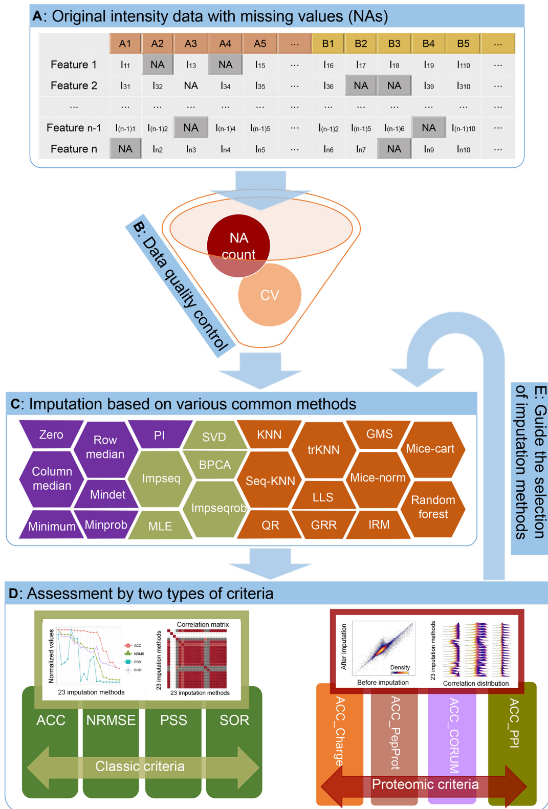
Figure 1. The overall workflow of NAguideR . (A) Uploading of original proteomics data with missing values (NAs). (B) Optional data quality control step for removing proteins/peptides with high proportion of NAs or large CV. (C) Missing value imputation based on the embedded methods. (D) Performance evaluation by multiple criteria (four classic criteria and four proteomic criteria). (E) The selection of well-performed imputation methods guided by the classic criteria and proteomic criteria.
