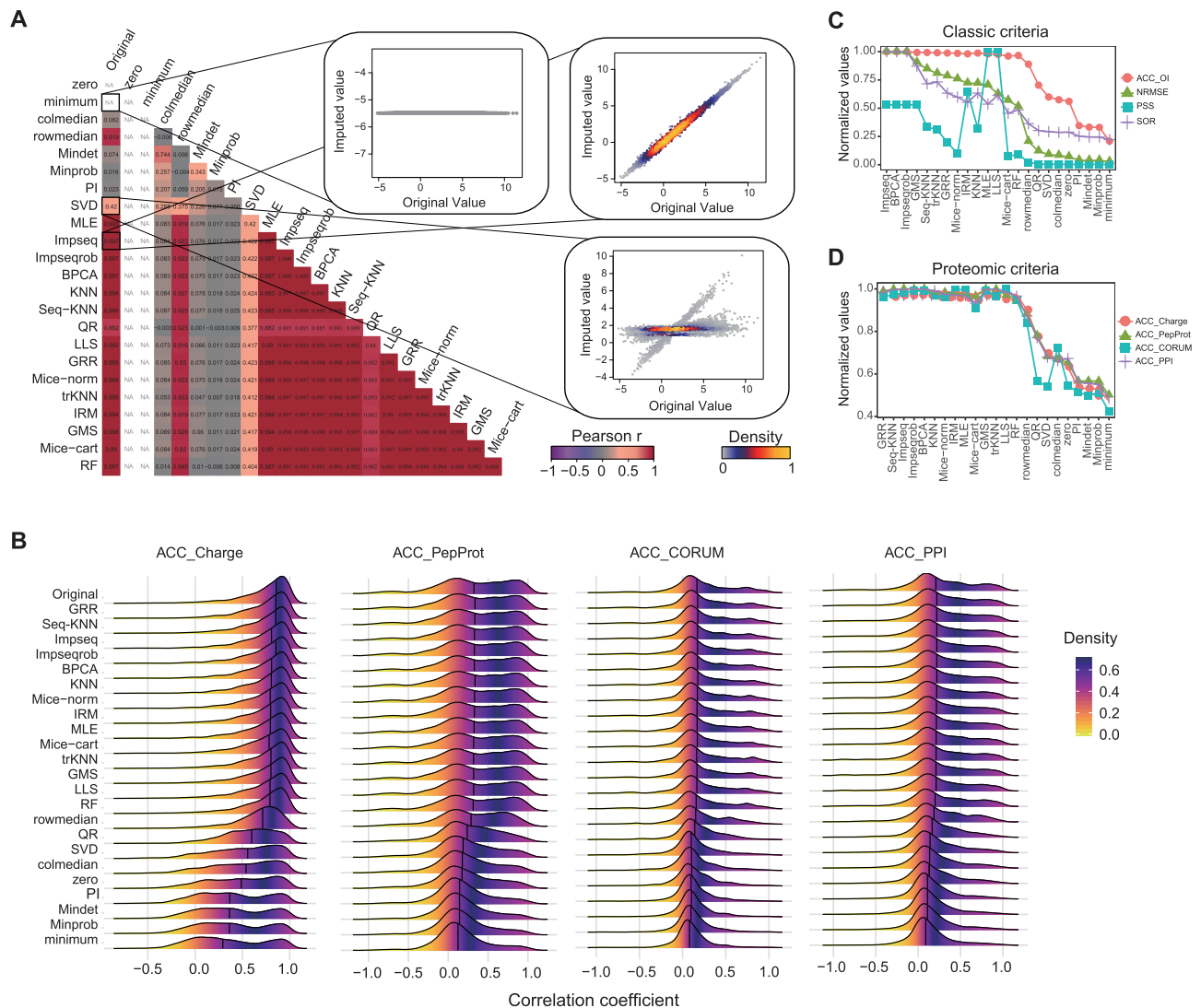
Figure 2. Systematic evaluation analysis of PhosDIA dataset. (A) Pearson correlation analysis of the original intensities and imputed intensities based on 23 methods. Density plots illustrate the correlation in detail between the original values and imputed values from minimum, SVD, and Impseq respectively as examples. NA in the correlation matrix means ‘No Result’ because the standard deviations of imputed values from zero and minimum method are equal to 0, and hence the cor function returns NA. (B) Comparison of the distribution of the correlation coefficient among original values and 23 imputation methods under the four proteomic criteria. The comprehensive scores distribution of 23 imputation methods under the four classic criteria (C) and four proteomic criteria (D). ‘Normalized values’ here means every score is divided by the corresponding maximum value.
