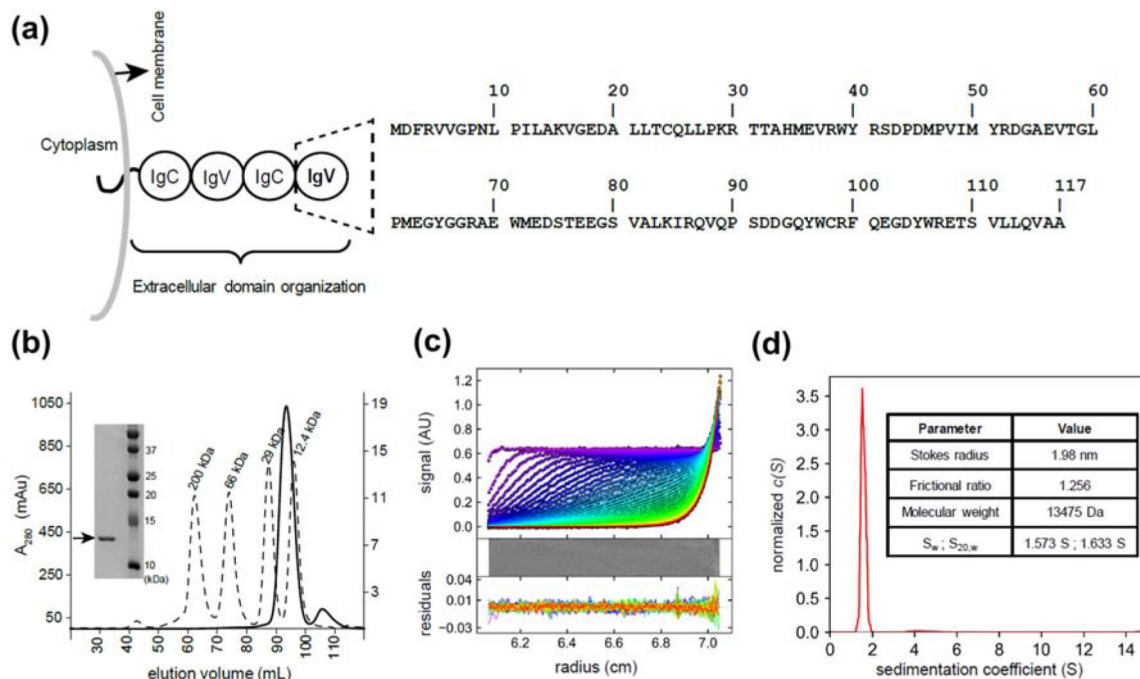
Figure 1: BTNL2 IgV domain exists as a monomer in solution
