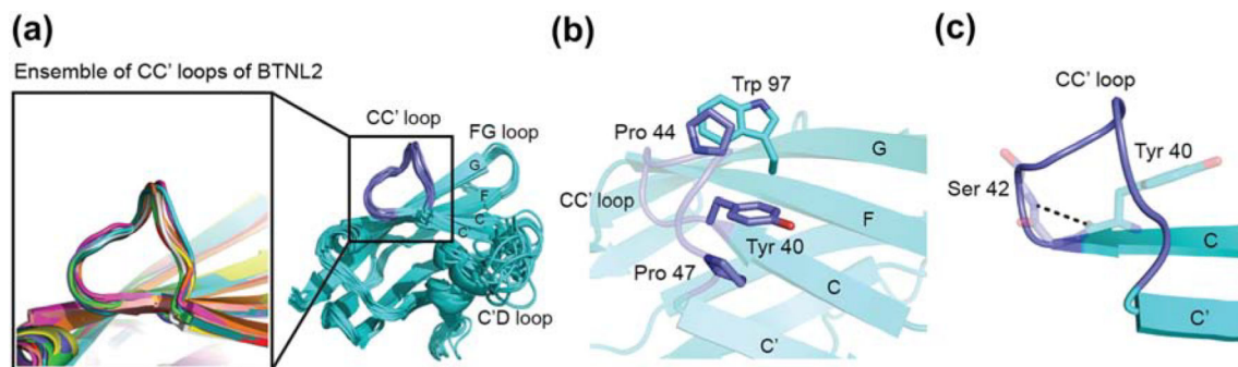
Figure 6: Non-canonical conformation of the CC' loop of BTNL2
