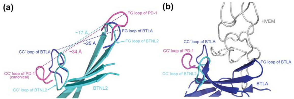
Figure 7: Non-canonical CC' loop reduces the surface area of the front face of BTNL2
