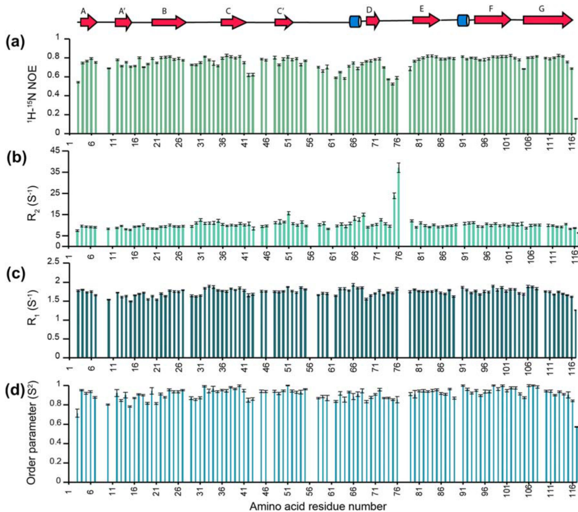
Figure 5: Backbone dynamics of BTNL2 IgV domain
