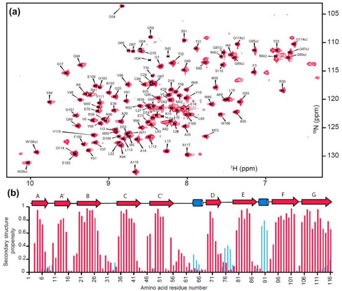
Figure 3: Backbone assignment and secondary structure propensity of BTNL2 IgV domain
