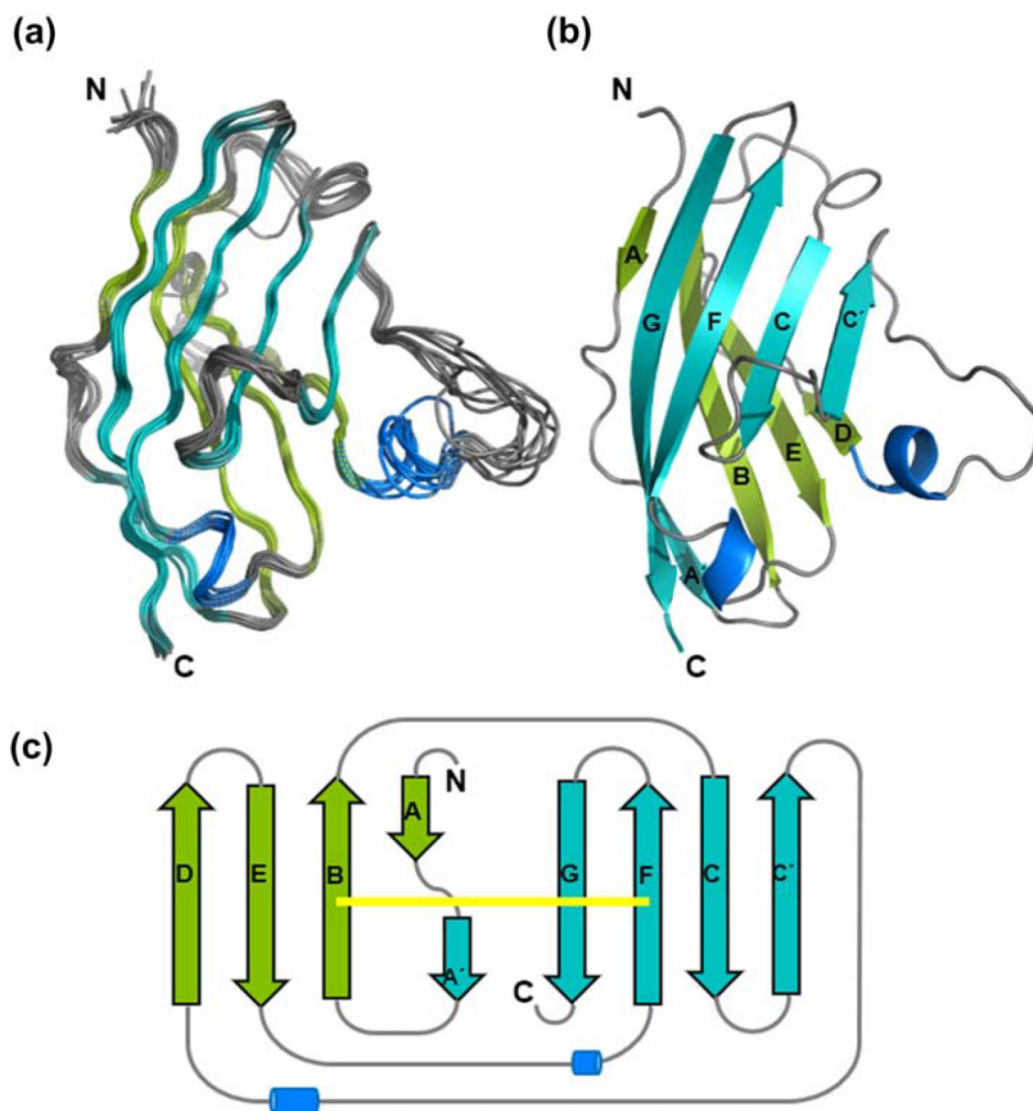
Figure 4: Solution NMR structure of BTNL2 IgV domain
