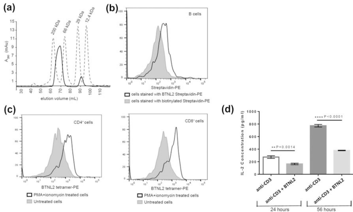
Figure 2: BTNL2 IgV domain binds to its putative receptor expressed on naïve B cells and in vitro activated CD4 + and CD8 + T cells
