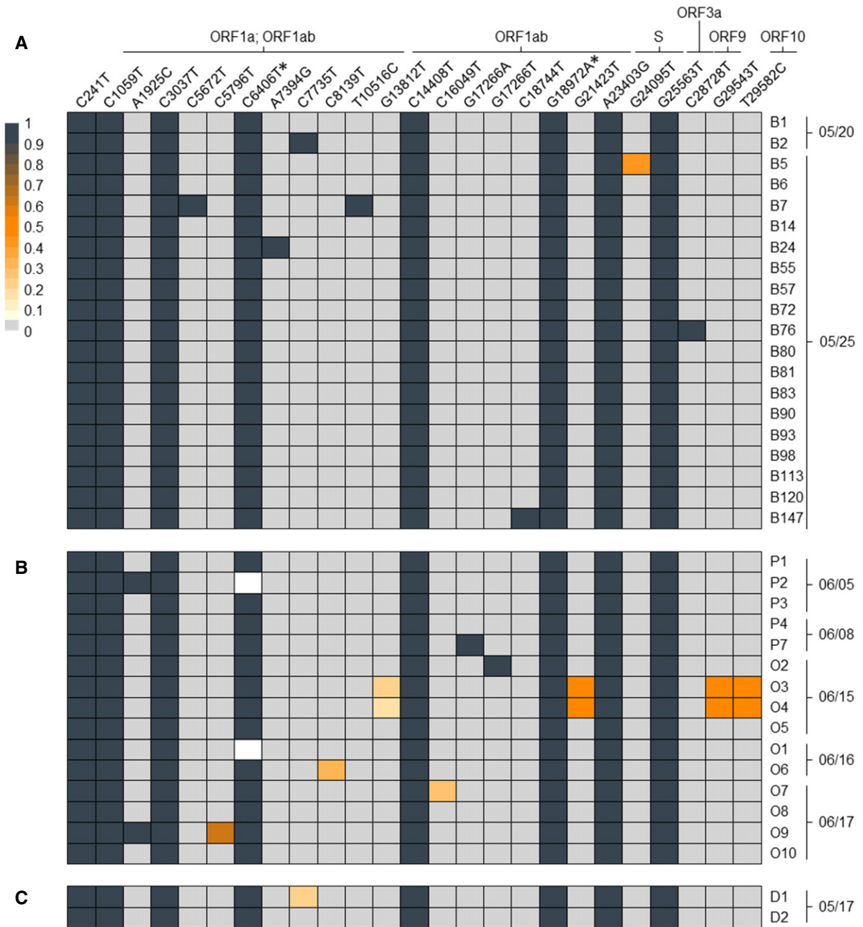
Figure 2. SARS-CoV-2 genotypes.
