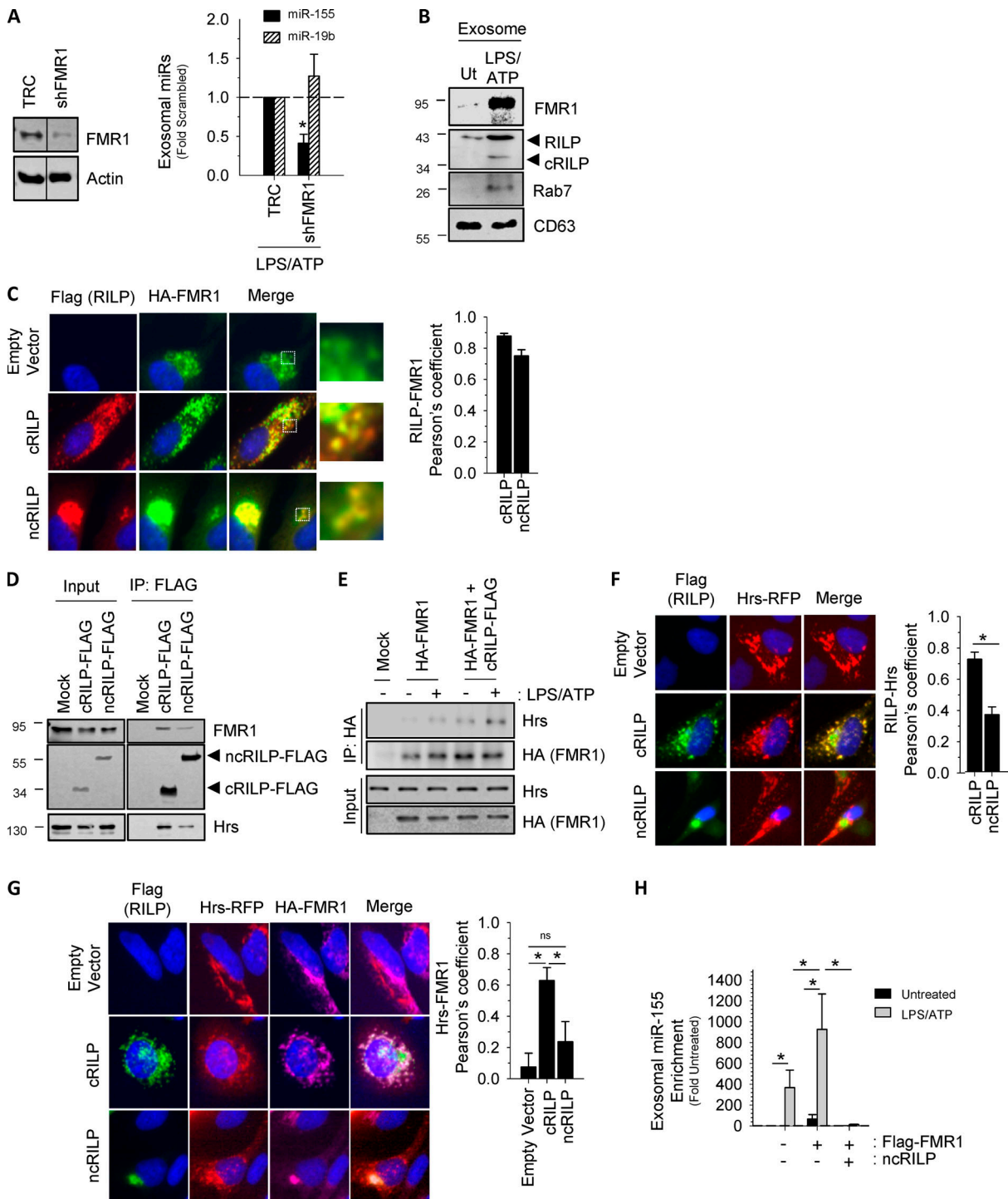
Figure 3. Identification of a cRILP-associated RBP. (A) Knockdown of candidate RBPs showing that shRNA to FMR1 blocks cRILP-associated miR-155 loading into exosomes after inflammasome activation by LPS and ATP, while not affecting miR-19b. TRC, empty vector control. (B) Western blot analysis of exosomes isolated from LPS/ATP-treated THP-1 cells shows that FMR1 is present in exosomes. These vesicles also contain cRILP and the RILP-associated GTPase, Rab7. Ut, untreated. (C) cRILP redistributes FMR1 throughout the cellular periphery. HeLa cells were transfected with HA-FMR1 with or without cRILP-Flag or ncRILP-Flag. HA-FMR1 (green) localizes loosely near the nucleus. Coexpression of cRILP (red) redistributes this localization toward the cell membrane, while ncRILP sequesters FMR1 in the mitotic center. Pearson's coefficients for n = 10-15 cells. (D) cRILP is more tightly associated with FMR1 and the ESCRT-related protein Hrs than is ncRILP. cRILP-Flag or ncRILP-Flag was expressed in HeLa cells and immunoprecipitated (IP) using Flag-tagged magnetic beads. (E) FMR1 associates with Hrs, and this association is increased when cRILP is expressed. HA-FMR1 was expressed alone or with cRILP-Flag and immunoprecipitated using HA-tagged magnetic beads. (F) cRILP relocates Hrs. HeLa cells were transfected with Hrs-RFP with or without cRILP-Flag or ncRILP-Flag. Hrs localizes in larger structures throughout the cytoplasm. Coexpression of cRILP (green) redistributes this localization into smaller puncta, extending toward the cell membrane. ncRILP has no effect on the distribution of Hrs. Pearson's coefficients for n = 12-15 cells. (G) cRILP induces the association between Hrs and FMR1. HeLa cells were transfected with Hrs-RFP and HA-FMR1 with or without cRILP-Flag or ncRILP-Flag. Coexpression of cRILP (green) enhances the
