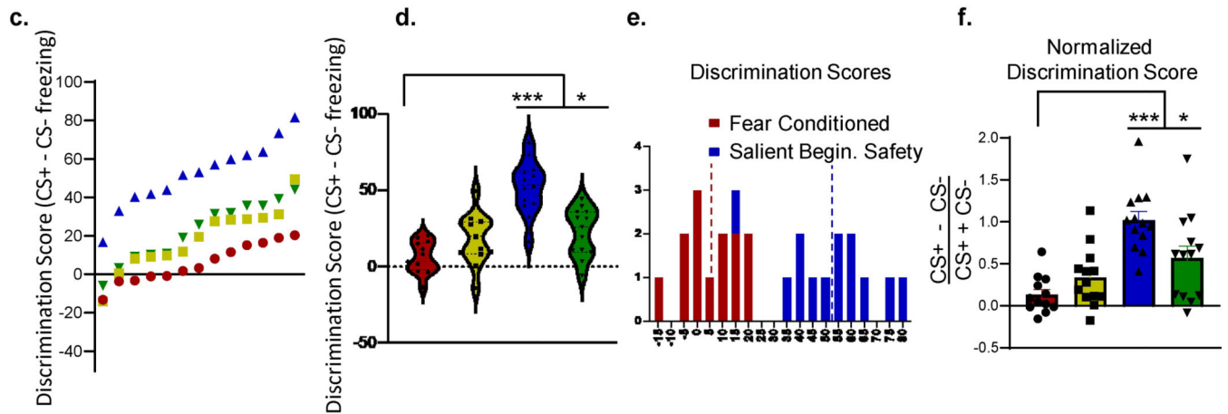
Figure 3: Salient Beginning Safety conditioned mice discriminate well during novel differential fear retrieval.
