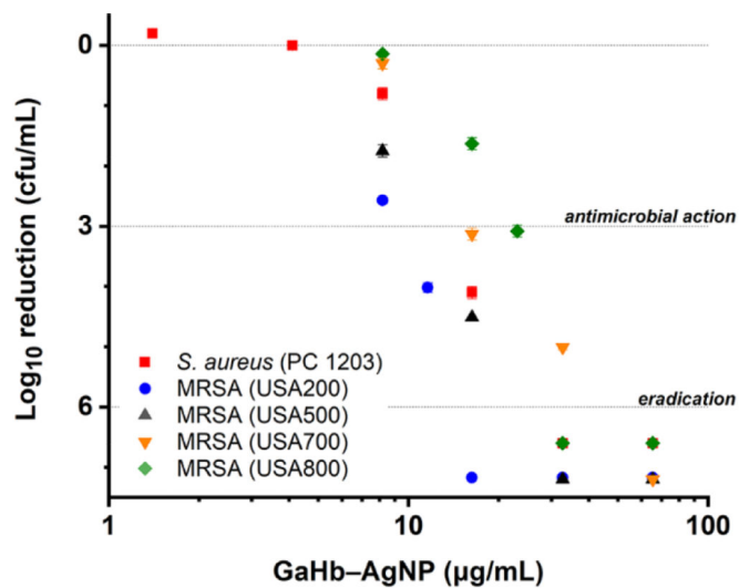
Figure 8. Photodynamic inactivation of S. aureus (PC 1203) and MRSA strains using 10-nm GaHb-AgNPs, following 15-min exposure to a 20-W CFL ( \lambda_{\text{max}} = 406 \text{ nm} ).
