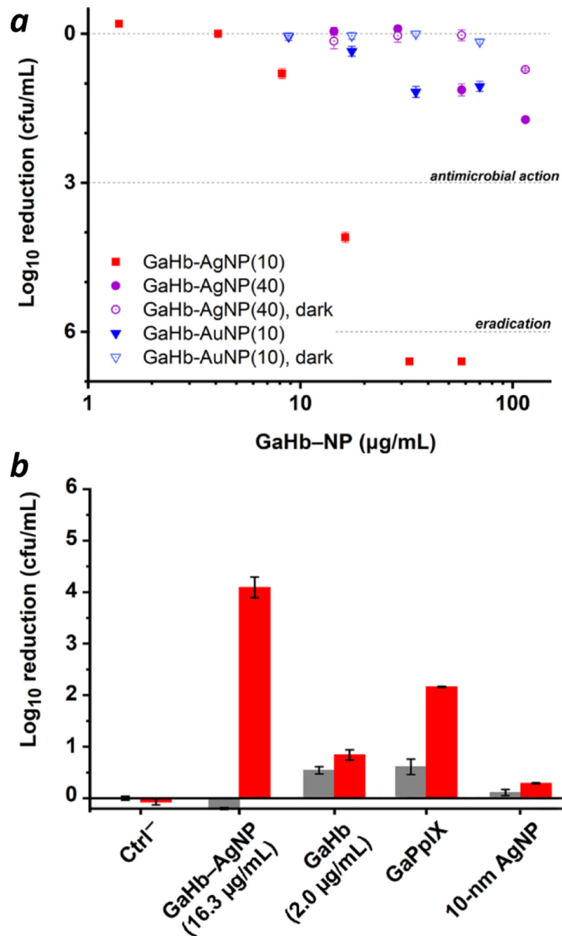
Figure 9. (a) Photodynamic activities of 10-nm GaHb-AuNPs (blue) and 40-nm GaHb-AgNPs (purple) on a per weight basis against S. aureus , following 15-min exposure to a 20-W CFL ( \lambda_{\max} = 406 nm). Activities for 10-nm GaHb-AgNPs (red) and GaHb-NPs without light (open symbols) included for comparison. (b) Photodynamic activities of various species (red bars) at equal loadings of GaPpIX (78 ng/mL). Dark toxicities (grey bars) included for comparison.
