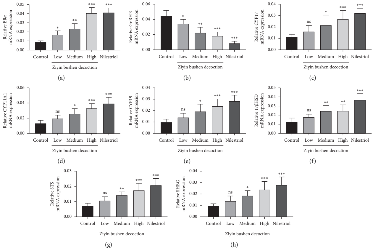
FIGURE 3: The Q-PCR results of ERα (a), GnRHHR (b), CYP17 (c), CYP11A1 (d), CYP19 (e), 17βHSD (f), STS (g), and SHGB (h) in ovarian tissue. * p < 0.05 , ** p < 0.01 , and *** p < 0.001 , compared with the control group; ns, no significant difference.
