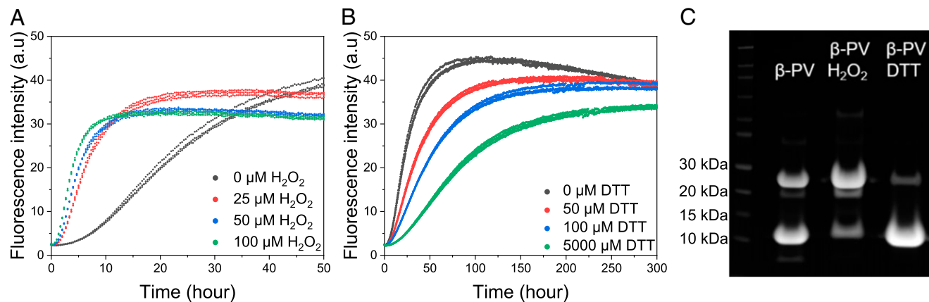
Fig. 2. (A and B) ThT fluorescence curves of 50 \mu M apo \beta -PV at 37 °C under quiescent conditions in 150 mM NaCl, 1 mM \text{CaCl}_2 , 5 mM EDTA, 25 mM Tris-HCl pH 7.4, and 0 to 100 \mu M \text{H}_2\text{O}_2 (A) or 0 to 5 mM DTT (B). (C) SDS/PAGE analysis of apo \beta -PV amyloid fibrils from ThT kinetic experiments with or without either 100 \mu M \text{H}_2\text{O}_2 or 100 \mu M DTT.
