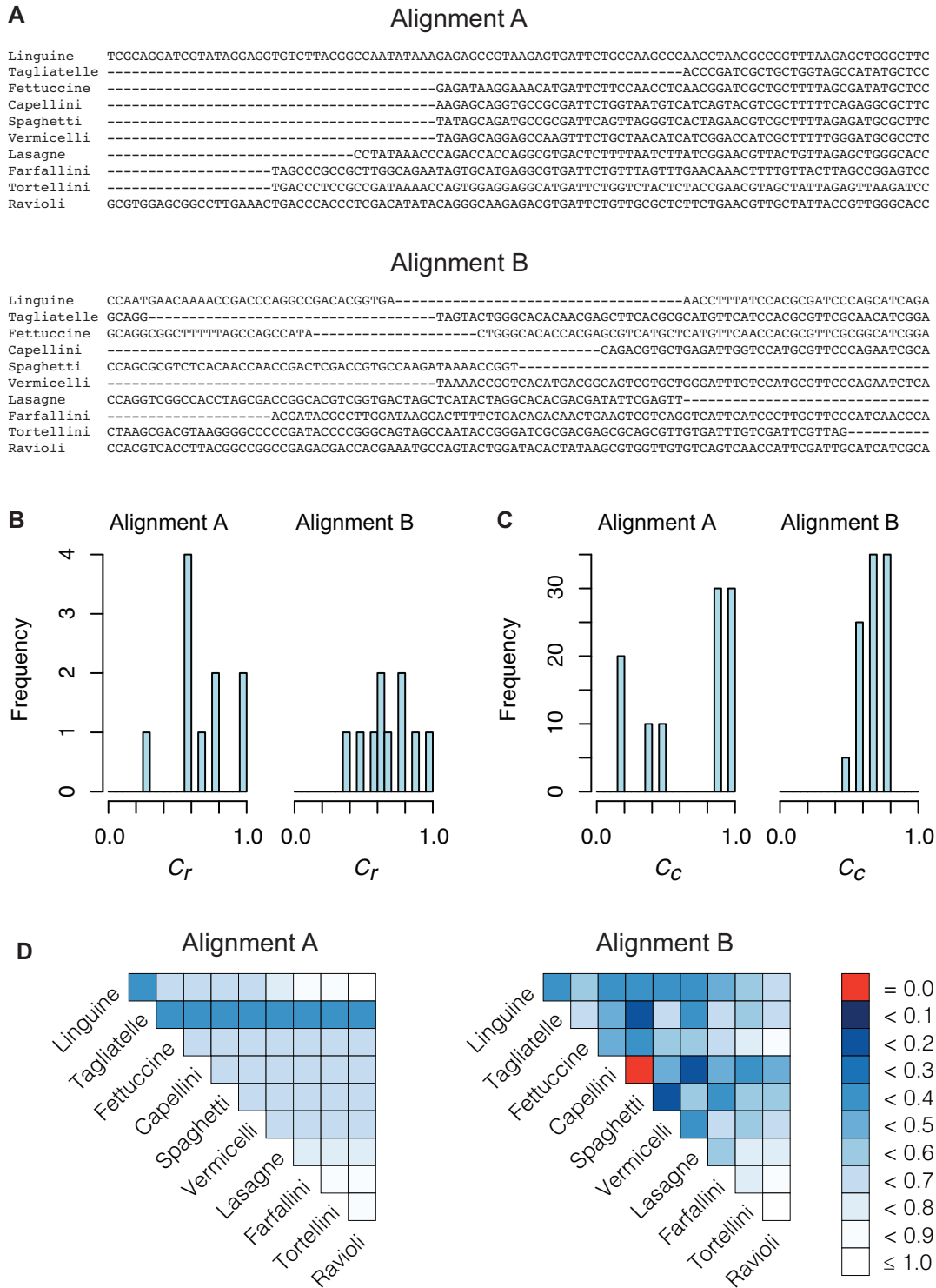
Figure 1. Example, based on two multiple sequences alignments (A), illustrating the corresponding distributions of completeness scores for rows (B), columns (C) and pairs of sequences (D).
