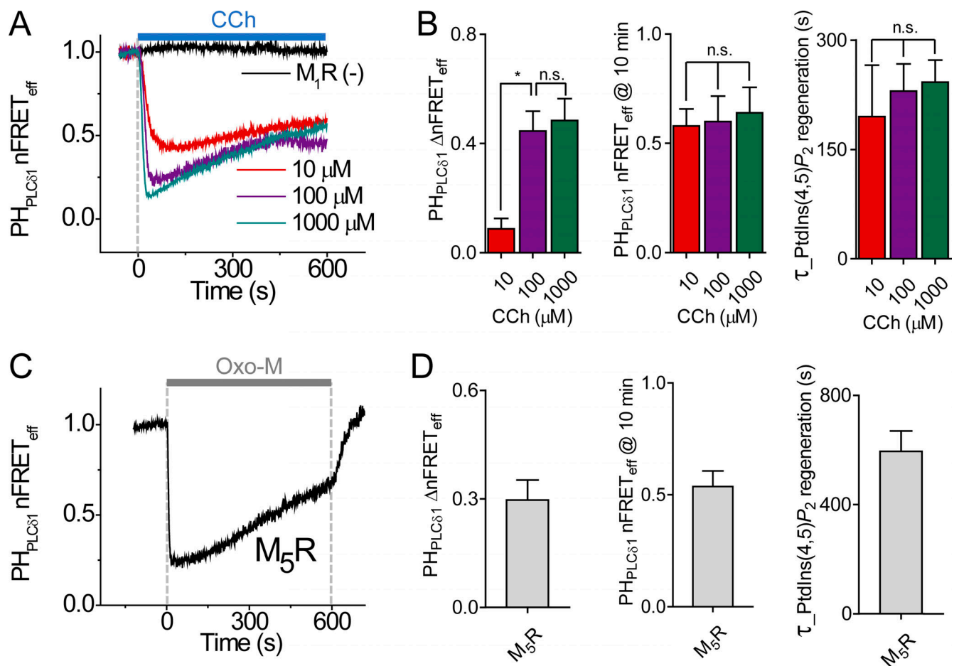
Figure S3. Comparison of PtdIns(4,5)P 2 regeneration during stimulation with different muscarinic agonists and receptors. (A) Time course of homologous nFRET eff between CFP- and YFP-tagged PH PLC \delta 1 domains during application of carbachol (light blue bar, CCh) for 10 min. Cells were transfected with the probes with or without (-) M 1 R. (B) Mean of \Delta nFRET_{eff} , nFRET eff after 10-min CCh stimulation, and the time constant of nFRET eff regeneration. 10 \mu M, n = 4 cells; 100 \mu M, n = 12 ; and 1,000 \mu M, n = 5 . (C) Time course of nFRET eff during application of 10 \mu M Oxo-M (gray bar) to cells expressing M 5 R. (D) Summary of \Delta nFRET_{eff} , nFRET eff at 10 min, and the time constant of nFRET eff regeneration for cells expressing M 5 R. n = 5 cells. *, P < 0.05 . n.s. not significant.
