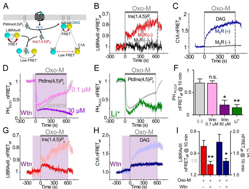
Figure 3. Exploring steps of the PI cycle by monitoring Ins(1,4,5) P_3 , DAG, and PtdIns(4,5) P_2 . (A) Schematic of Ins(1,4,5) P_3 and DAG indicators. LIBRAVIII has CFP and YFP at opposite termini of an Ins(1,4,5) P_3 binding domain. (B) Time course of intramolecular LIBRAVIII nFRET eff during a 10-min stimulation with 10 \mu M Oxo-M (gray bar) in cells with or without expression of M 1 R. Note inverted y axis for LIBRAVIII since FRET is reduced by binding of Ins(1,4,5) P_3 to this receptor. (C) Time course of homologous nFRET eff between CFP- and YFP-tagged C1A domains with or without expression of M 1 R. CFP- and YFP-tagged C1A domains detect DAG at the PM and increase their FRET when DAG increases at the PM. (D) Comparison of pretreatment with 0.1 \mu M or 30 \mu M Wtn (shaded area) on PtdIns(4,5) P_2 regeneration during M 1 R stimulation by 10 \mu M Oxo-M (gray, control; pink, 0.1 \mu M Wtn; and purple, 30 \mu M Wtn). (E) Effect of 2-h pretreatment with 10 mM Li + -enriched solution on regeneration of PtdIns(4,5) P_2 (gray, control; green, Li + ). (F) Mean PtdIns(4,5) P_2 regeneration measured as homologous nFRET eff of CFP- and YFP-tagged PH PLC \delta 1 at 10 min of Oxo-M treatment. Control, n = 6 cells; 0.1 \mu M Wtn, n = 9 ; 30 \mu M Wtn, n = 9 ; Li + , n = 4 . (G) Wtn (shaded area) limits Ins(1,4,5) P_3 regeneration during M 1 R activation as measured with LIBRAVIII (pink, control; red: 30 \mu M Wtn). (H) Wtn depresses DAG production as measured with C1A probes (aqua, control; blue, 30 \mu M Wtn). (I) Mean Wtn effect on production of Ins(1,4,5) P_3 (red bars) and DAG (blue bars) measured as nFRET eff at 10 min of Oxo-M treatment. Ins(1,4,5) P_3 : control, n = 4 cells and Wtn, n = 6 ; DAG: control, n = 9 and Wtn, n = 6 cells. *, P < 0.05 ; **, P < 0.005 . n.s., not significant.
