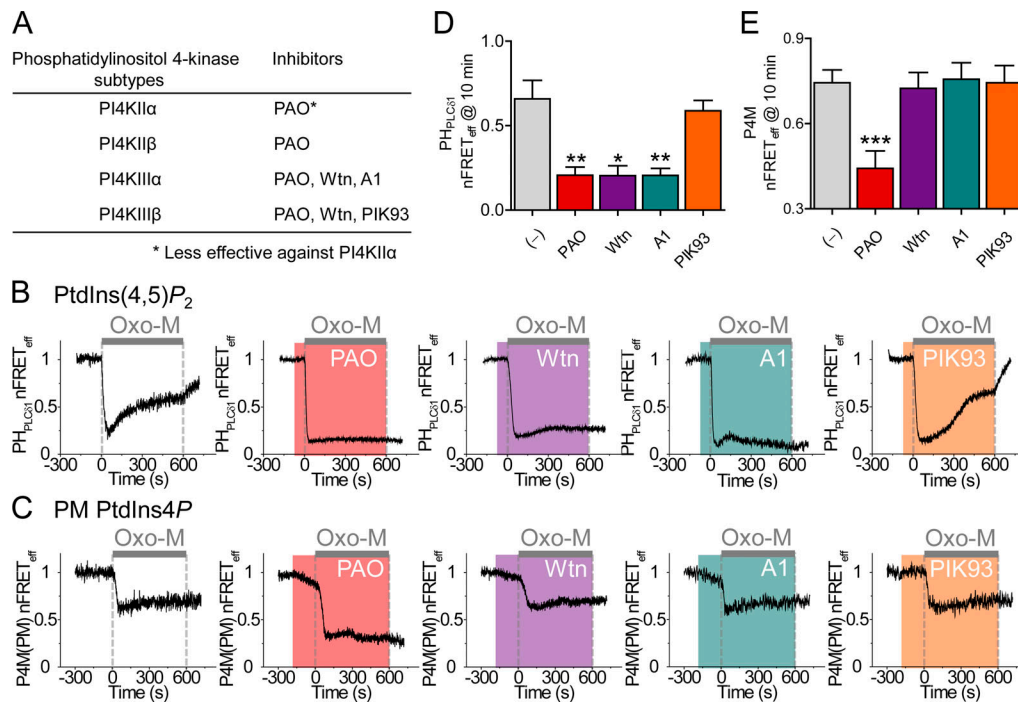
Figure 5. Depression of PtdIns(4,5)P 2 regeneration by PI4KIII \alpha inhibitors. (A) Specificity of inhibitors for PI4K subtypes. (B) Time course of PtdIns(4,5)P 2 during 10- \mu M Oxo-M application (gray bar) measured from homologous FRET between CFP- and YFP-tagged PH PLC \delta 1 probes in cells pretreated (shaded areas) with different PI4K inhibitors (30 \mu M PAO, 30 \mu M Wtn, 30 nM A1, and 300 nM PIK93). (C) Time course of PtdIns4P in the PM measured from heterologous FRET between P4M-CFP and Lyn-YFP in cells pretreated (shaded areas) with different PI4K inhibitors. (C-E) Mean PI4K inhibitor effects on the regeneration of PtdIns(4,5)P 2 (D) and on PM PtdIns4P (E) as measured with FRET indicators at 10 min of Oxo-M stimulation. PtdIns(4,5)P 2 : control, n = 4 cells; PAO, n = 5 ; Wtn, n = 5 ; A1, n = 8 ; and PIK93, n = 9 . PtdIns4P: control, n = 25 ; PAO, n = 15 ; Wtn, n = 15 ; A1, n = 12 ; and PIK93, n = 7 cells. *, P < 0.05 ; **, P < 0.005 ; ***, P < 0.001 .
