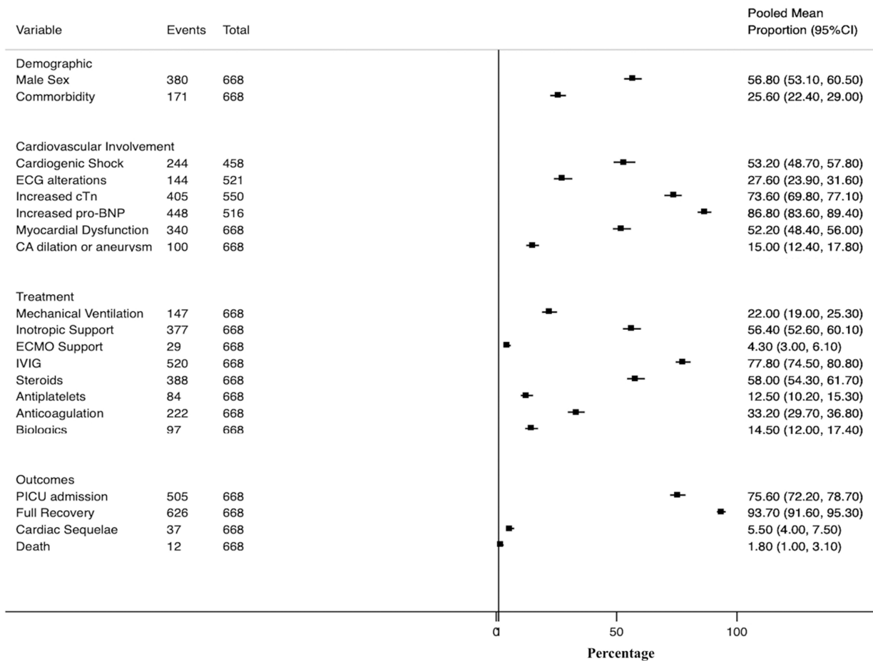
Figure 1 Forest plot that summarizes the pooled mean proportion of the cardiovascular characteristics of children with pediatric multisystem inflammatory syndrome associated with coronavirus disease-2019. Multiple separate meta-analyses were conducted. Considering the high likelihood of between study variance, a random effects model was used. Continuity correction for total zero events studies was performed to include these in the meta-analysis as recommended. Pooled data were presented with 95%CI and displayed using forest plots. Heterogeneity within studies was assessed using I^2 statistics. For all the factors analyzed, the P value for heterogeneity was determined to be > 0.10 and the I^2 values were < 50\% (adequate heterogeneity between studies).
