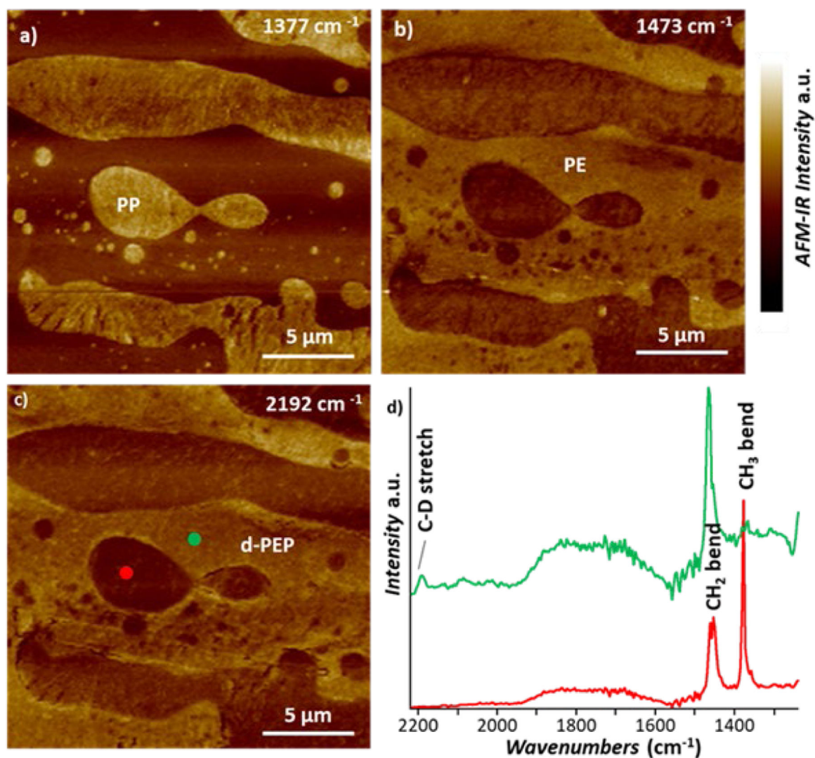
Fig. 4. AFM-IR images of a three-component blend made by polyethylene (PE), polypropylene (PP) and deuterated polyethylene-propylene copolymer (d-PEP) obtained at (a) 1377\text{ cm}^{-1} ( \text{CH}_3 bending of PP), (b) 1473\text{ cm}^{-1} ( \text{CH}_2 bending of PE) and (c) 2192\text{ cm}^{-1} ( \text{CD}_2 stretching of d-PEP). (d) AFM-IR spectra obtained at the color-coded locations marked in panel-d. The data show that the d-PEP copolymer partitions in the PE phase but does not mix with the PP phase. 58 These AFM-IR experiments were obtained in ringdown mode. This figure has been adapted from M. A. Rickard (ref. 58) with permission from Elsevier, copyright 2020. 58
