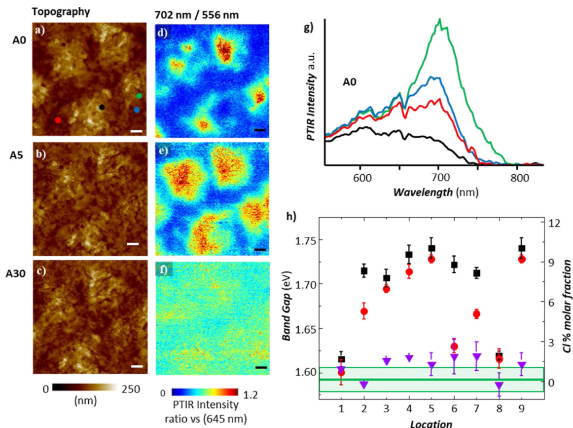
Fig. 5. \text{CH}_3\text{NH}_3\text{PbI}_{3-x}\text{Cl}_x perovskite AFM topography maps (a–c) and corresponding absorption ratio (702 nm/556 nm, i.e. 1.77 eV/2.23 eV) maps (d–f) as a function of annealing: A0, as prepared (a and d), A5, 5 min annealing at 95 °C (b and e), A30, additional annealing for 5 min at 95 °C and for 20 min and at 110 °C (c and f). The red and blue tones indicate Cl-poor and Cl-rich regions, respectively. All scale bars are 1.0 \mu\text{m} . (g) PTIR spectra obtained at the color-coded locations in panel-a for the as prepared sample. (h) Local bandgap (left axis) and local Cl% content (right axis) obtained by linearly fitting the spectra at 9 locations as a function of annealing: as prepared sample (A0, black squares), A5 (red circles), A30 (purple triangles). Upon annealing the local bandgap and \text{Cl}^- content decreases at all locations, approaching the bandgap of the \text{CH}_3\text{NH}_3\text{PbI}_3 phase (green horizontal line). The light green rectangle and error bars represent a single standard deviation in the calculation of the local bandgap due to the linear fitting of nanoscale the absorption spectra. 41 These AFM-IR experiments were obtained in ringdown mode. Adapted with permission from J. Chae et al. , Nano Lett. , 2015, 15 , 8114–8121. Copyright (2015) American Chemical Society.
