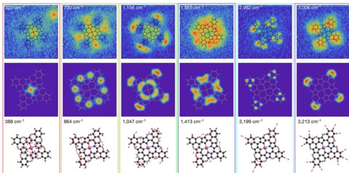
Fig. 16. TERS images (top row) of individual CoTPP molecule allows for visualization of vibrational normal modes (middle and bottom rows). Reproduced from Lee et al. , Nature , 2019, with permission from Nature Publishing Group.
