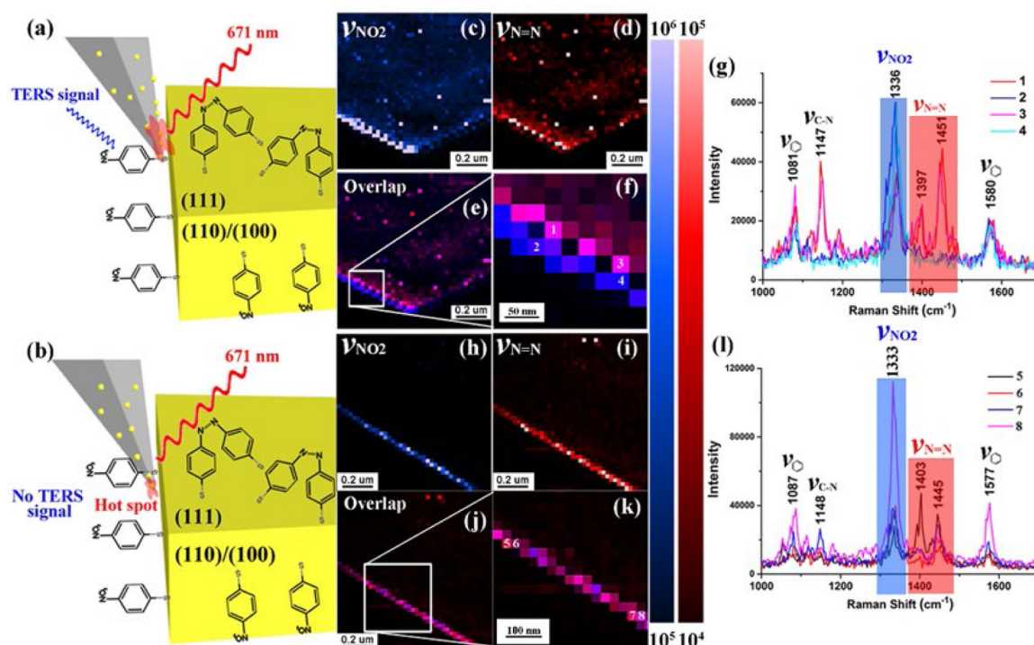
Fig. 17. TERS imaging of the facet-dependent reduction of pNTP catalyzed by Au microplates. (a and b) Proposed schemes showing the hot-spot located at both the shaft and apex (a) and only at the apex (b) of the TERS probe. (c, d) and (h, i) High resolution TERS images of the distribution of -\text{NO}_2 (c and h) and \text{N}=\text{N} groups (d and i) obtained with 3D TERS active and inactive probes respectively. (e and j) Corresponding overlap of \text{NO}_2 and \text{N}=\text{N} images (c and d for e; h and i for j). (f and k) Zoomed-in TERS images of the white rectangle position in (e) and (j), respectively. (g and l) Typical TERS spectra extracted from the marked position in (f) and (k). Reprinted with permission from Wang and Kurouski, J. Phys. Chem. C , 2018. Copyright (2018) American Chemical Society.
