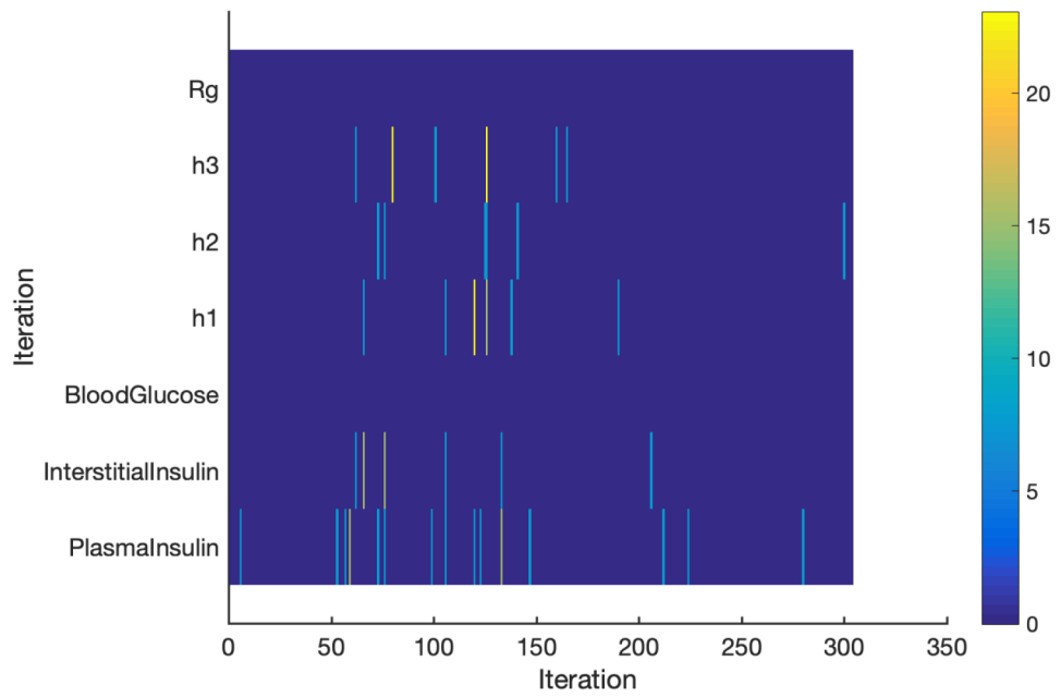
Figure 3. Percentage map of the constraint violations, where each lower-bound constraint is represented by a row. At each iteration, the percentage of particles that violated a constraint is color-coded, with yellow representing the largest proportion of constraint violations.
