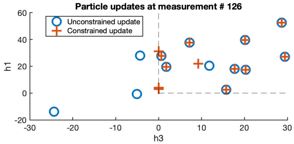
Figure 2. Particle updates at a given time-step (here, measurement 126) are shown using a traditional Kalman gain versus using the constrained optimization. The black lines denote lower bound constraints on the states h_1 and h_3 .
