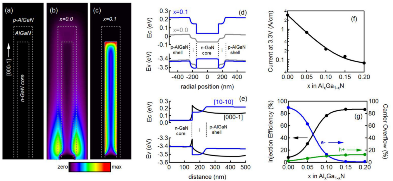
Figure 1. 2D models of core-shell AlGaIn/GaN NW LEDs forward biased at 3.3 V and with varying Al mole fraction in the shell layer. The simulated structure is shown in (a) along with the resulting spontaneous recombination profiles for (b) x=0.0 and (c) x=0.1 . Band diagrams comparing x=0.0 and x=0.1 in the radial direction are shown in (d) and band diagrams comparing the axial and radial directions for x=0.1 are shown in (e). The (f) simulated current integrated over the 2D contact surfaces at 3.3 V forward bias and (g) injection efficiency/carrier overflows are shown as a function of Al mole fraction.
