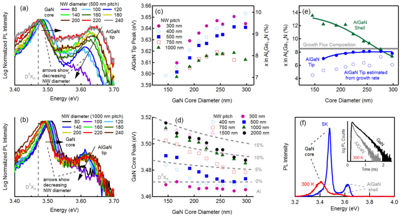
Figure 4. Diameter-dependent PL spectra of AlGaN/GaN core-shell NWs obtained at 5K for (a) 500 nm and (b) 1000 nm pitch spacings. Peak positions are shown for the (c) AlGaN tip and corresponding tip Al mole fraction calculated via bowing parameters and for the (d) GaN core along with calculated strain-induced shifts ( E_{A,B} ) for varying shell Al mole fraction (dashed lines). The overall tip/shell Al mole fractions determined by PL and by growth rate analysis are shown in (e) for NW arrays with 1000 nm pitch spacing. PL spectra obtained at 300 K and 5 K and time-resolved PL decay curves obtained at 300 K (inset) are shown in (f) for NWs from the 1000 nm pitch spacing and 160 nm nominal hole diameter array.
