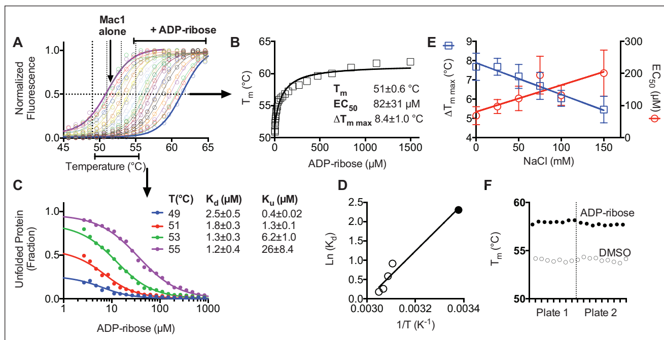
Figure 1. DSF assay optimization. (A) Normalized SPYRO Orange fluorescence in the presence of 4.75 \mu\text{M} Mac1 protein at various temperatures in the presence of indicated concentrations of ADPr. Data are fit to eq 1 using nonlinear regression with GraphPad Prism. (B) T_m values obtained from direct fitting to eq 1. Data are fit to eq 2. (C) Isothermal analysis 9 of percent unfolded protein at each indicated temperature. Data are fit to eq 3 with indicated constants. Uncertainties are standard errors of the curve fits. (D) Van't Hoff plot of estimated K_d values from C (open circles) and the K_d for ADPr binding to Mac1 that was previously determined at 23 °C using isothermal titration calorimetry (filled circle). 3 (E) ADPr titrations in 20 mM MOPS pH buffer supplemented with indicated NaCl concentrations. Plotted are best-fit \Delta T_{m \max} (squares, left y axis) and EC_{50} (circles, right axis). Error bars mark standard errors in the curve fits. (F) T_m values for positive (500 \mu\text{M} ADPr) and negative (DMSO only) controls from two different 96-well plates ( Z' factor = 0.72).
