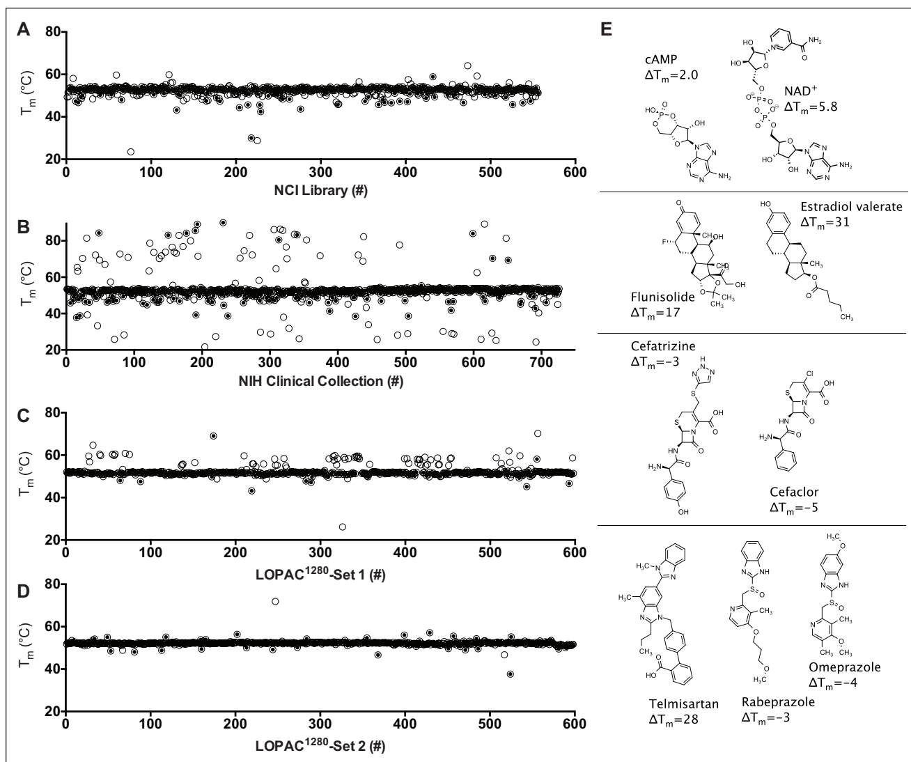
Figure 2. DSF screens of FDA-approved drugs and drug-like compounds for SARS-CoV-2 Mac1 ligands. T_m values calculated by fitting melting curves to eq 1 (open circles) obtained for Mac1 in the presence of each compound in (A) the NCI library, (B) the NIHcc, and (C,D) the LOPAC 1280 . Assays yielding a “typical” melting curve, as defined by the TSA-CRAFT algorithm, are noted (filled circles). (E) Selected hit compounds separated based on chemotype: nucleotides, steroids, \beta -lactam antibiotics, and benzimidazoles.
