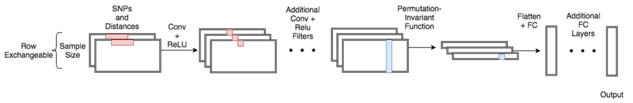
Figure 1: A cartoon schematic of the exchangeable architecture for population genetics.
