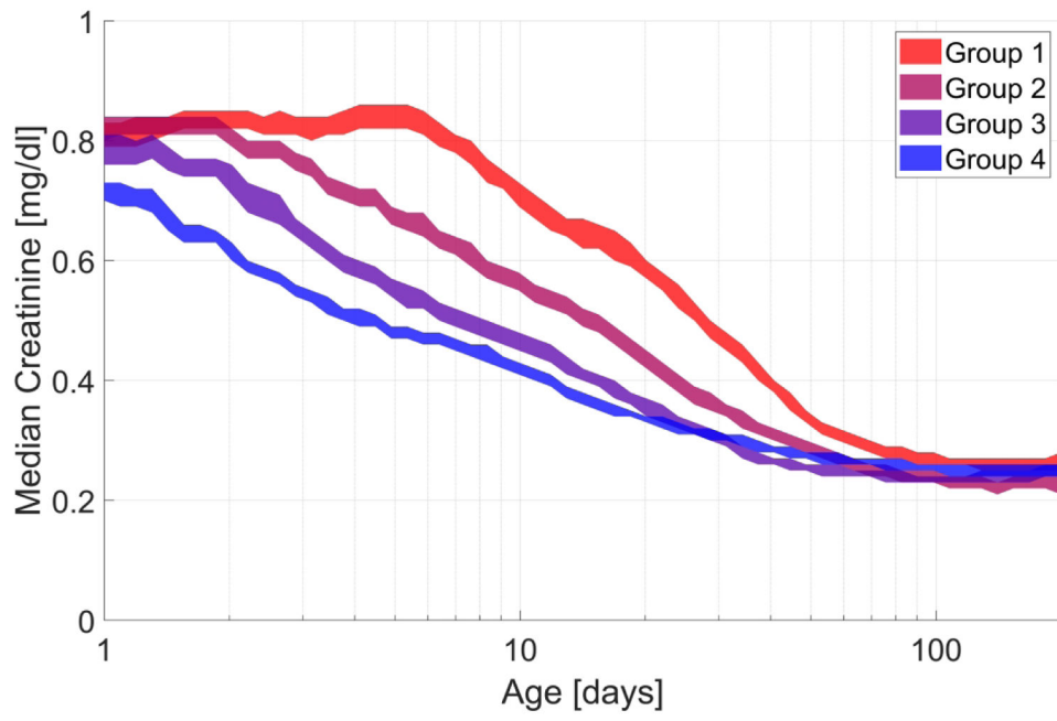
Figure 2. 95% Confidence region for moving median for each group
