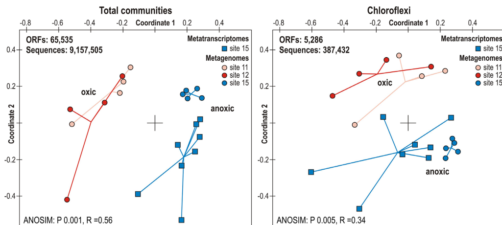
Figure 6. Non-metric dimensional scaling (NMDS) plot for all three sites based on metagenomes and metatranscriptomes. (Left) NMDS plot for all three sites based on all ORFs from the metagenomes (circles) and metatranscriptomes (squares) for the entire microbial communities. (Right) NMDS plot for all three sites based on annotated protein-encoding ORFs from the metagenomes (circles) and metatranscriptomes (squares) assigned to Chloroflexi.
