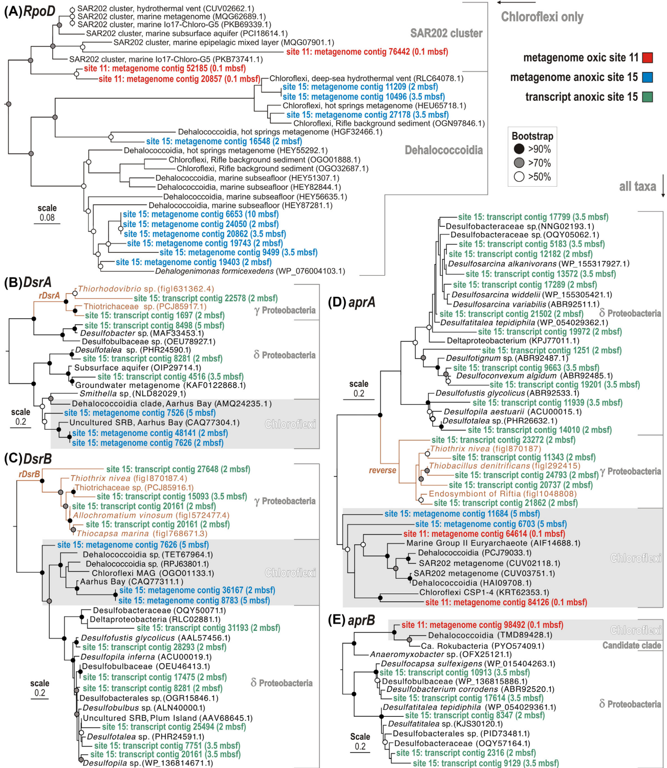
Figure 4. Phylogenetic analysis of predicted proteins encoded by selected marker genes in the metagenomes and metatranscriptomes from oxic and anoxic sites, based on RAxML using BLOSUM62 as the evolutionary model. (A) Phylogeny of Chloroflexi RNA polymerase sigma factor ( RpoD ) ORFs (619 aligned amino acid sites). (B) Phylogeny of all DsrA and rDsrA ORFs detected (466 aligned amino acid sites). (C) Phylogeny of all DsrB and rDsrB ORFs detected (433 aligned amino acid sites). (D) and (E) Phylogenies of all aprA and aprB ORFs detected (754 and 157 aligned amino acid sites, respectively). All phylogenies were conducted with 100 bootstrap replicates, circles on the nodes indicate support values (black > 90%, gray > 70%, white > 50%). Dsr : dissimilatory sulfite reductase; rDsr : reverse dissimilatory sulfite reductase; apr : adenylylsulfate reductase; A and B: alpha and beta subunits.
