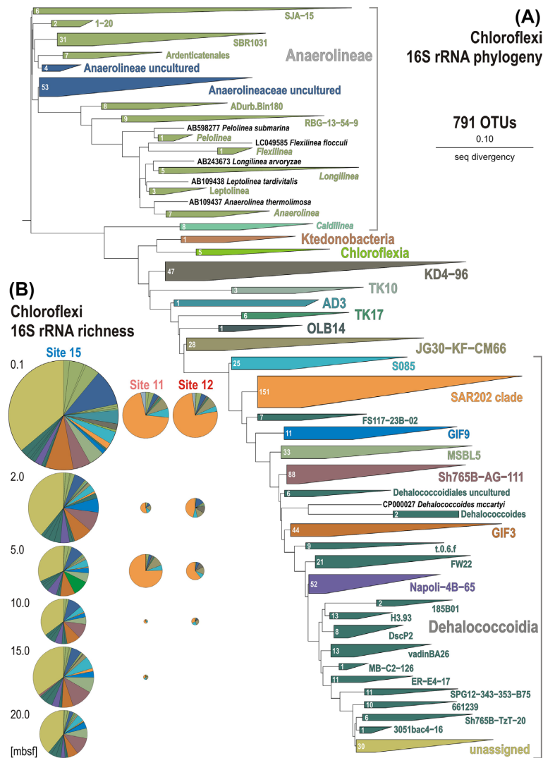
Figure 2. Phylogenetic analysis of 16S rRNA genes (V4 hypervariable region). (A) Phylogenetic tree obtained for all operational taxonomic units (OTUs) assigned to Chloroflexi in this study. (B) Pie charts displaying 16S rRNA gene richness of the whole assemblage of Chloroflexi for each of the three sites and at each sediment depth. The radii of pie charts are proportional to the number of OTUs. The clockwise color coding in the pie charts matches that of the phylogenetic tree from top to bottom, and bar charts from left to right (Fig. 1).
