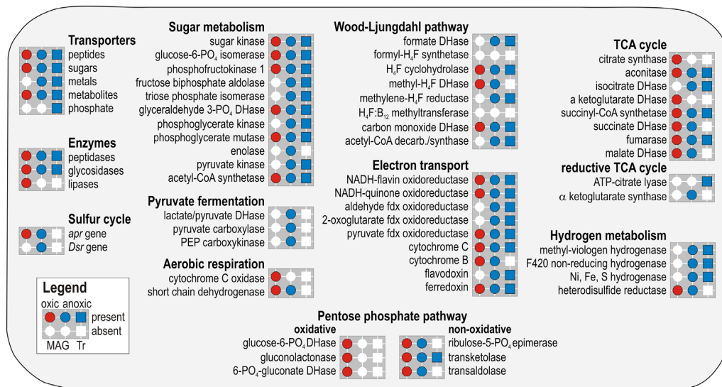
Figure 5. Presence and absence of Chloroflexi assigned predicted proteins as detected in the present metagenomes and metatranscriptomes. Presence (colored) or absence (white) of metabolic functions (circles) and expressed genes (squares) identified in the metagenomes and metatranscriptomes at the oxic (red) and anoxic (blue) sites across all depths sampled. Presence/absence of substrate transporters, catabolytic enzymes, apr and Dsr genes are shown on the left hand side. Metabolic pathways listed correspond to sugar metabolism, pyruvate fermentation, aerobic respiration, Wood-Ljungdahl pathway, electron transport, tricarboxylic acid (TCA) cycle, hydrogen metabolism and oxidative and non-oxidative pentose phosphate pathway. The complete list of ORFs with assignment and coverage is available as Supplementary Data.
