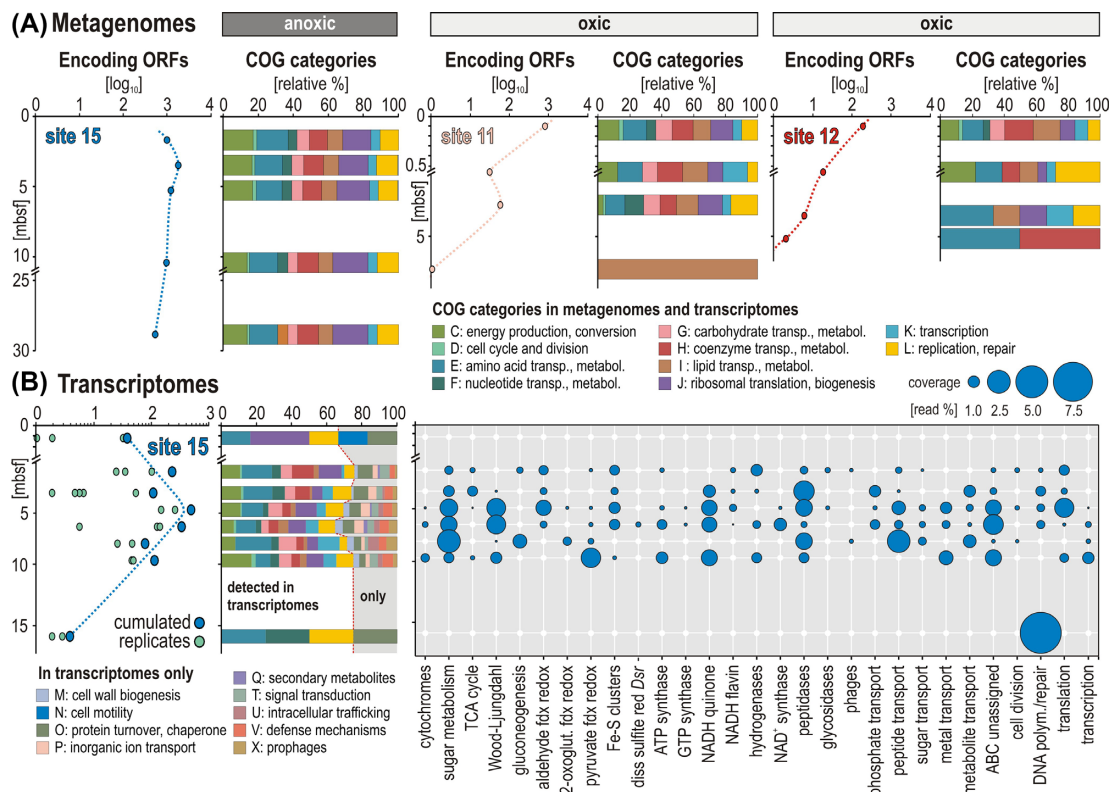
Figure 3. Open reading frames (ORFs) assigned to Chloroflexi, their COG categories and metabolic potential obtained from metagenomes and metatranscriptomes. (A) Number of annotated protein-encoding ORFs obtained from metagenomes and attributed to Chloroflexi with sediment depth at the three sites; relative abundances of different COG categories and metabolic functions obtained from metagenomes at the three sites. (B) Number of annotated protein-encoding ORFs obtained from the metatranscriptomes and attributed to Chloroflexi with sediment depth at the anoxic site; relative abundances of different COG categories and metabolic functions that are expressed at the anoxic site [read % coverage].
