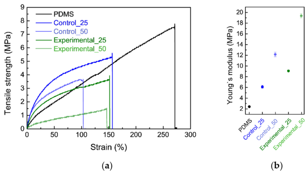
Figure 1. Tensile stress-strain curves (a) and Young's modulus (b) of different bioelastomers (PDMS, Control_25, Control_50, Experimental_25, and Experimental_50).
