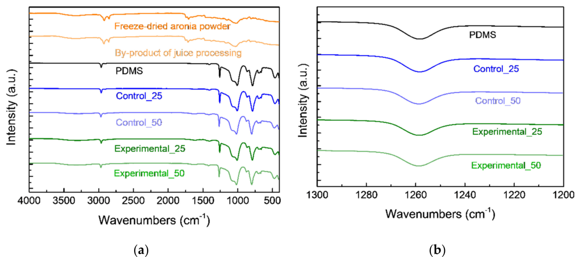
Figure 4. (a) Attenuated total reflectance–Fourier transform infrared spectroscopy (ATR-FTIR) spectra of aronia freeze-dried powder, aronia juice processing by-products, PDMS (0 wt%), Control_25, Control_50, Experimental_25, and Experimental_50; (b) details of Si-CH 3 bands of bioelastomers.
