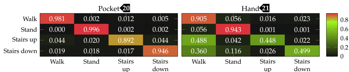
Figure 26. Final confusion matrices for the best-performing configuration (LDA, 2.5 s windows, 5 dimensions, two-channel acceleration) of the statistical features approach, for pocket-case and hand-case using an SVM classifier. Each row represents the actual class, each column the classification.
