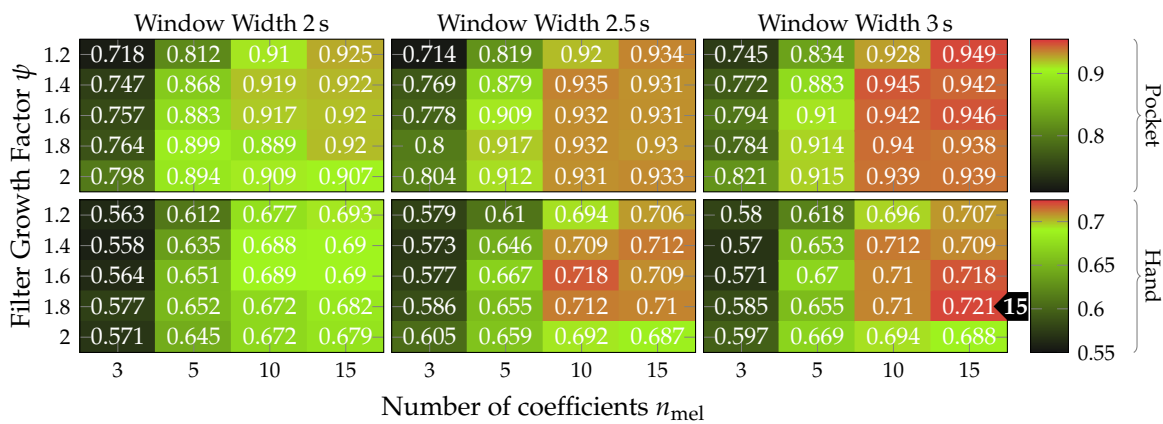
Figure 22. Results of benchmarks done for the hyperparameters n_{mel} and \psi , controlling number, as well as growth of filters in the used MFCC filter-bank respectively, for both pocket-case and hand-case.
