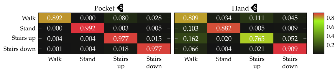
Figure 16. Final confusion matrices for the best-performing configuration (PCA, 5 dimensions, 2s windows, raw acceleration) of the analytical transformations approach for pocket-case and hand-case using an SVM classifier. Each row represents the actual class, each column the classification results.
