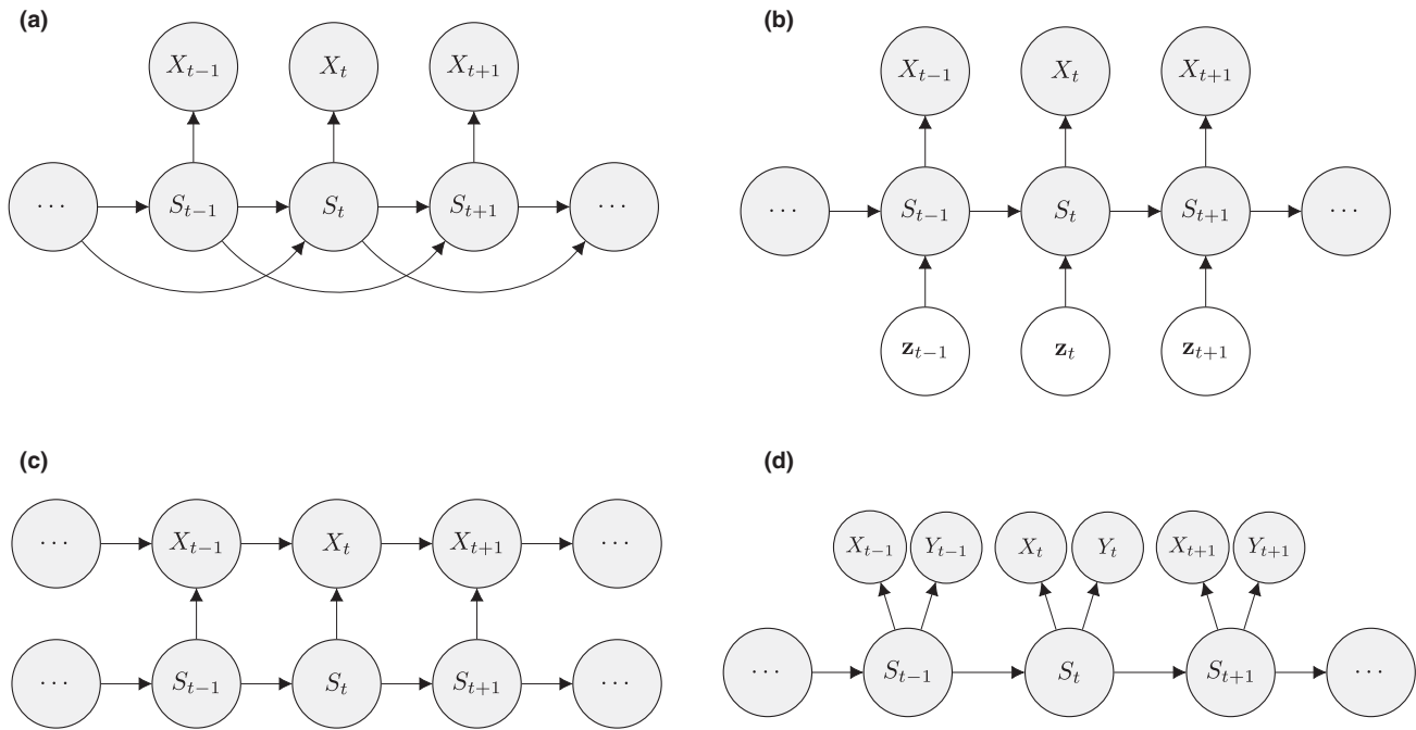
Figure 4 Graphical models associated with different extensions of the basic HMM formulation: (a) state sequence with memory order 2; (b) influence of covariate vectors z_1, \dots, z_T on state dynamics; (c) observations depending on both states and previous observations; (d) bivariate observation sequence, conditionally independent given the states.
