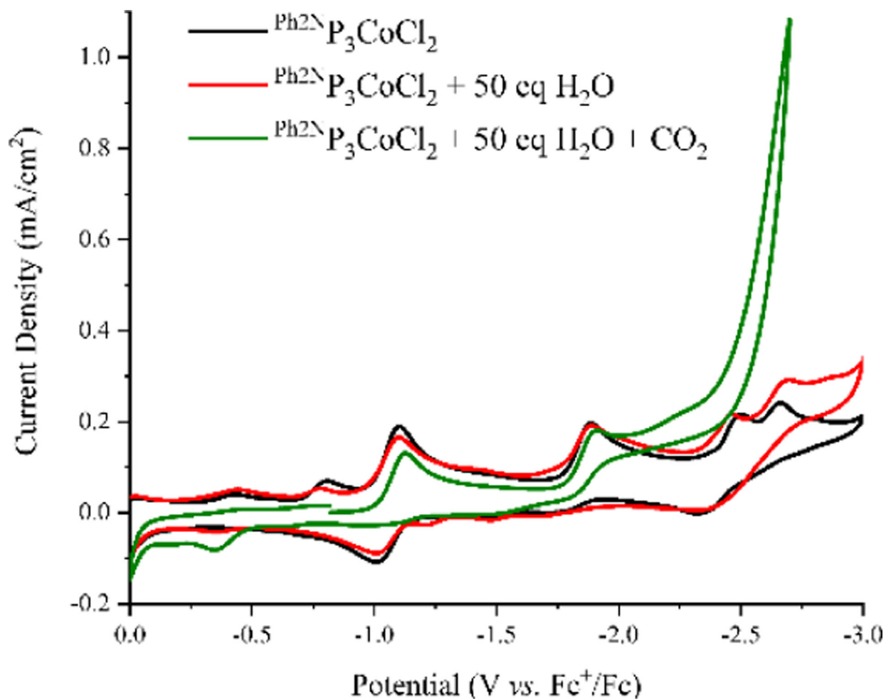
Figure 3. Cyclic voltammograms of 1 mM Ph 2 N-P 3 CoCl 2 under various conditions. (black) : under N 2 ; (red) : in the presence of 50 eq H 2 O; (green) : in the presence of 50 eq H 2 O and CO 2 . Conditions: GC working electrode, 0.1 M TBAPF 6 electrolyte in MeCN solvent, scan rate of 0.06 V/s, initial scan is positive
