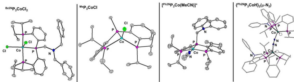
Figure 1. 50% Thermal ellipsoid plot of several complexes. All hydrogen atoms not located in the difference map are removed for clarity. Only the cation of [(\text{Ph}_2\text{N})\text{P}_3\text{Co}(\text{MeCN})][\text{BArF}] is shown.
