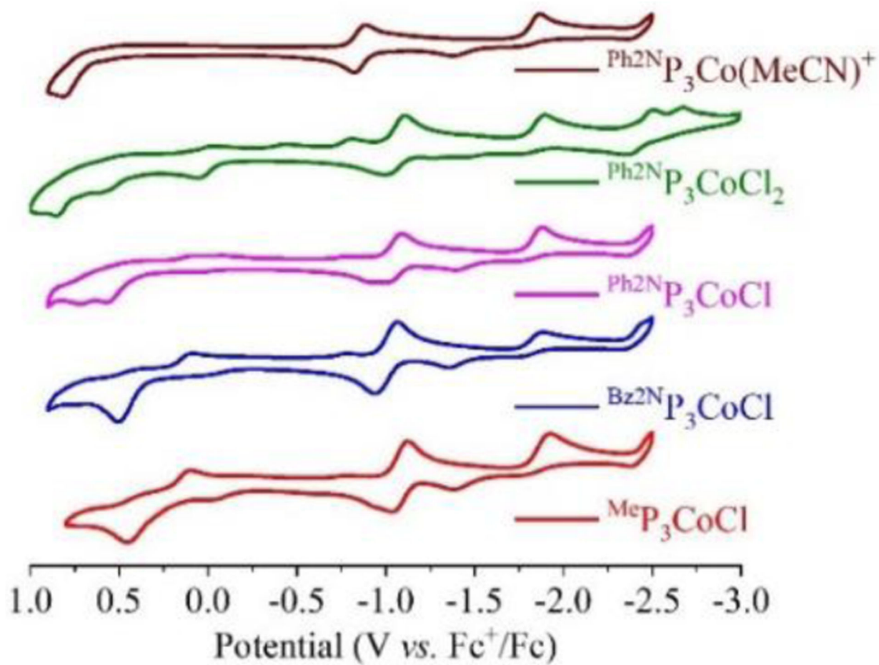
Figure 2. Cyclic voltammograms of the various Co complexes. Conditions: GC working electrode, 0.1 M TBAPF 6 electrolyte in MeCN. Initial scan is in the positive direction.
