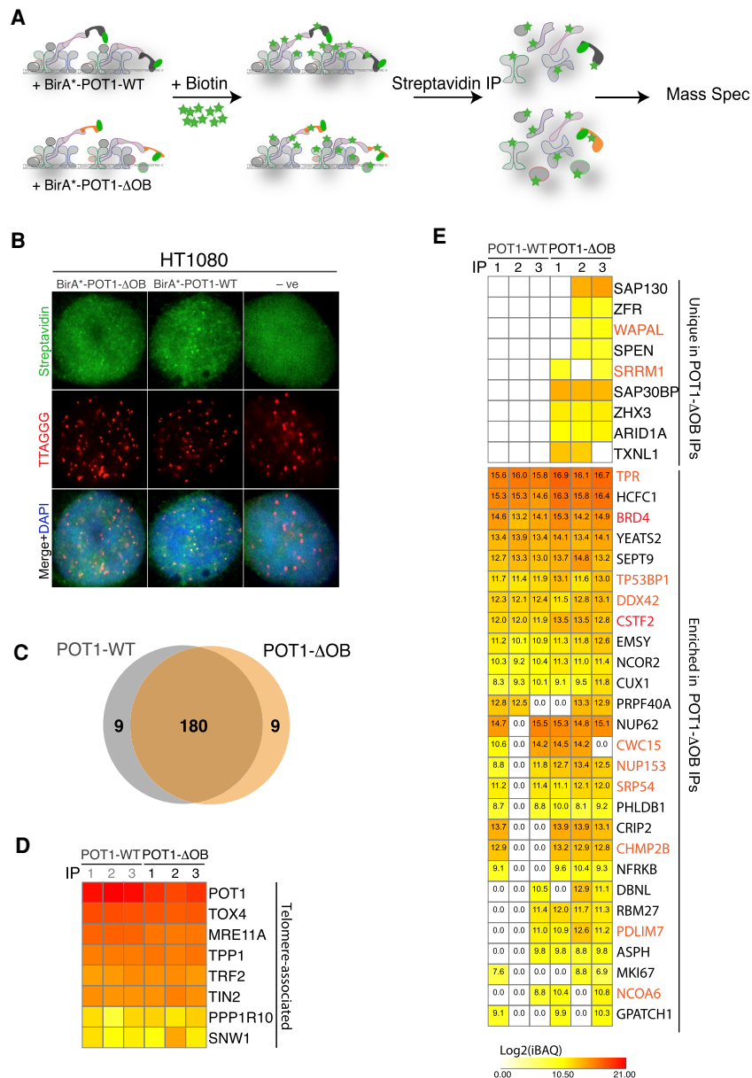
Figure 2. Proteomic analysis of the telomere interactome in cells expressing a POT1 OB-fold mutation. (A) Schematic of the biotinylation (BirA*) purification scheme to characterize the telomere proteome in cells expressing BirA*-POT1-WT and BirA*-POT1-ΔOB. BirA* covalently attaches biotin to lysine residues on vicinal proteins. Labeled proteins are recovered by streptavidin immunoprecipitation (IP) and identified using liquid chromatography–mass spectrometry. IPs were performed in triplicate for each POT1 variant. (B) Indirect immunofluorescence (IF) for streptavidin (green) coupled with fluorescence in situ hybridization for telomeres (FISH) (red) in HT1080 cells with the indicated treatment and following overnight incubation with excess biotin. Cells expressing an empty vector were used as negative control for the staining. (C) Venn diagram of the overlap between POT1-WT and POT1-ΔOB hits identified in two or more IPs. (D) Heat map of the log 2 transformed intensity-based absolute quantification (iBAQ) values for telomere-associated proteins recovered in cells expressing BirA*-POT1-WT or BirA*-POT1-ΔOB. n = 3 independent IPs. (E) Heat map of the log 2 transformed iBAQ values of proteins enriched at telomeres in POT1-ΔOB cells. (Top) Proteins uniquely present in two or more IPs in POT1-ΔOB-expressing cells. (Bottom) iBAQ values for proteins with ≥50% enrichment (≥0.6 in log 2 ) in two or more IPs in cells expressing POT1-ΔOB compared with those expressing POT1-WT. Values were compared in a paired manner (i.e., IP#1 for POT1-WT with IP#1 for POT1-ΔOB). Highlighted in red are enriched proteins that have been identified as SL candidates in the genome-wide screen (Supplemental Table S1).
