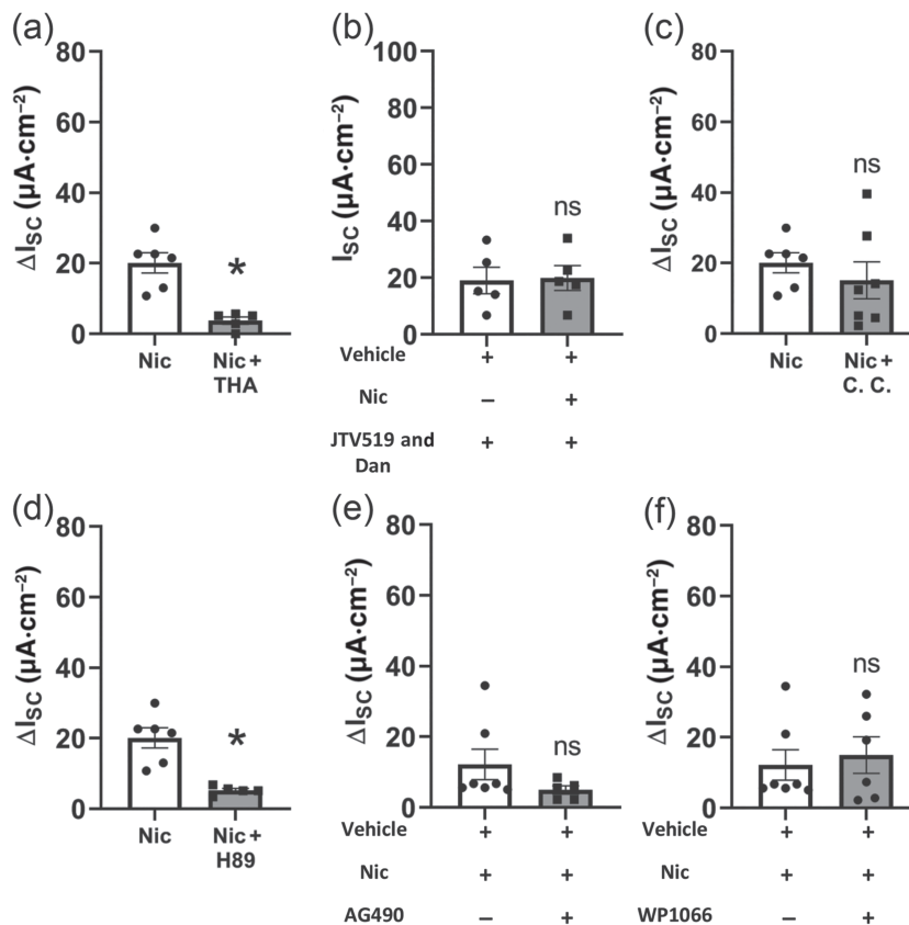
FIGURE 4 Downstream signalling involved in the nicotine-induced activation of transepithelial ion transport in mouse trachea. (a) Application of 1- \mu M thapsigargin (THA, apical, n = 5 ), an inhibitor of the \text{Ca}^{2+} -ATPase in the endoplasmic reticulum, significantly reduced the nicotine effect (100 \mu M, apical, \Delta I_{\text{SC}} , * P < 0.05 ). (b) In the presence of the ryanodine receptor antagonist JTV519 and dantrolene (each 10 \mu\text{mol}\cdot\text{L}^{-1} , apical), nicotine (100 \mu\text{mol}\cdot\text{L}^{-1} , apical) had no effect on I_{\text{SC}} (ns, not significant; n = 5 ). (c) The protein kinase C (PKC) inhibitor chelerythrine chloride (CC, 5 \mu\text{mol}\cdot\text{L}^{-1} , apical and basolateral, n = 7 ) did not influence the nicotine effect (100 \mu\text{mol}\cdot\text{L}^{-1} , apical, \Delta I_{\text{SC}} ; ns, not significant). (d) In the presence of the protein kinase A (PKA) inhibitor H-89 (10 \mu\text{mol}\cdot\text{L}^{-1} , apical and basolateral, n = 5 ), the current induced by nicotine (100 \mu\text{mol}\cdot\text{L}^{-1} , apical, \Delta I_{\text{SC}} , * P < 0.05 ) was significantly reduced. (e) Application of the JAK2 inhibitor AG 490 (50 \mu\text{mol}\cdot\text{L}^{-1} , apical and basolateral, n = 5 ) did not lead to a significant change of the nicotine effect (100 \mu\text{mol}\cdot\text{L}^{-1} , apical, \Delta I_{\text{SC}} , * P < 0.05 ). (f) Application of the STAT3 inhibitor WP1066 (10 \mu\text{mol}\cdot\text{L}^{-1} , apical, n = 6 ) did not influence the nicotine effect (100 \mu M, apical, \Delta I_{\text{SC}} ; ns, not significant)
