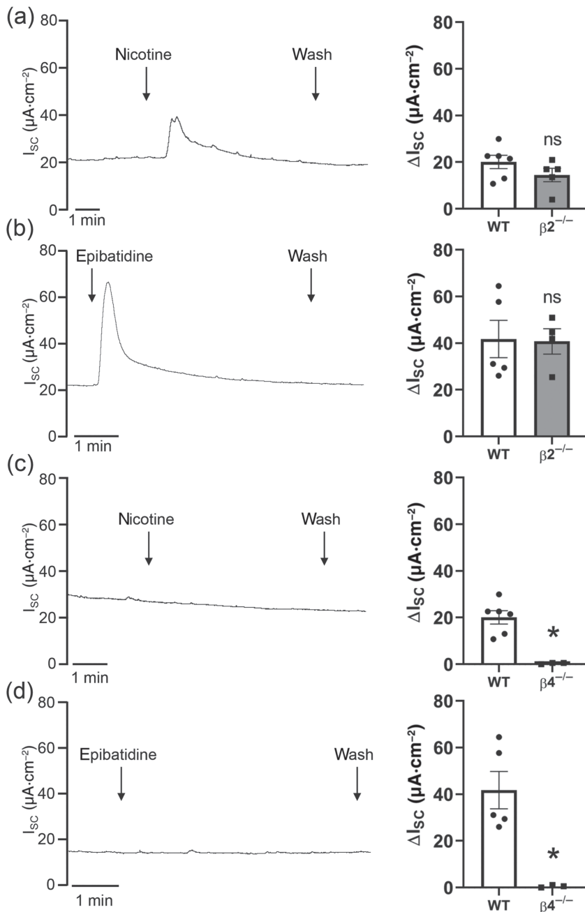
FIGURE 3 Effect of nicotine or epibatidine on transepithelial ion transport in \beta 2 - or \beta 4 -deficient mice. (a) Apical application of nicotine ( 100 \mu\text{mol}\cdot\text{L}^{-1} ) in \beta 2^{-/-} mice resulted in a transient reversible increase in the short circuit current ( I_{sc} ). Representative current trace. (b) The nicotine-induced peak ( \Delta I_{sc} ) in \beta 2^{-/-} mice was similar to wild-type (WT) mice ( n = 5 ; ns, not significant). (c) Apical application of epibatidine ( 1 \mu\text{mol}\cdot\text{L}^{-1} ) in \beta 2^{-/-} mice resulted in a transient reversible increase in I_{sc} . Representative current trace. (d) The epibatidine-induced peak ( \Delta I_{sc} ) was similar in WT and \beta 2^{-/-} mice ( n = 5 ; ns, not significant). (e) Apical application of nicotine ( 100 \mu\text{mol}\cdot\text{L}^{-1} ) in \beta 4^{-/-} mice did not influence I_{sc} . Representative current trace. (f) The nicotine-induced peak ( \Delta I_{sc} ) in \beta 4^{-/-} mice was significantly reduced compared to WT mice ( n = 5 , *P < 0.05 ). (g) Apical application of epibatidine ( 1 \mu\text{mol}\cdot\text{L}^{-1} ) in \beta 4^{-/-} mice had no effect on I_{sc} . Representative current trace. (h) The epibatidine-induced peak ( \Delta I_{sc} ) was significantly reduced in \beta 4^{-/-} mice compared to WT mice ( n = 5 , *P < 0.05 )
