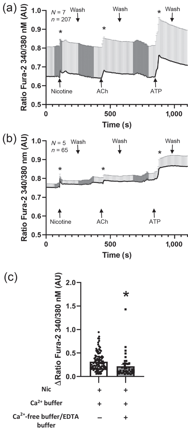
FIGURE 5 \text{Ca}^{2+} imaging and immunohistochemistry experiments of tracheal epithelial cells of wild-type mice. (a) Application of nicotine, ACh, or ATP significantly increased [\text{Ca}^{2+}]_i compared to baseline in the presence of \text{Ca}^{2+} -containing external solution (normal Tyrode's). N , number of animals; n , number of cells. (b) Application of nicotine, ACh, or ATP increased [\text{Ca}^{2+}]_i compared with baseline in the presence of \text{Ca}^{2+} -free external solution. N , number of animals; n , number of cells. (c) The nicotine-induced [\text{Ca}^{2+}]_i was significantly reduced in \text{Ca}^{2+} -free buffer compared to extracellular \text{Ca}^{2+} -containing solution (Tyrode's)
