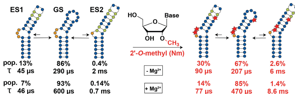
Figure 6. Summary of the effect of Nm on GS-ES exchange in the presence and absence of Mg 2+ . Bulge nucleotides are shown in orange. Nucleotides that transition from being unpaired in GS to paired in the ES are shown in green. Red stars indicate the Nm-modified residues. Pop and \tau refer to the population and lifetime of the conformational state (GS, ES1 or ES2).
