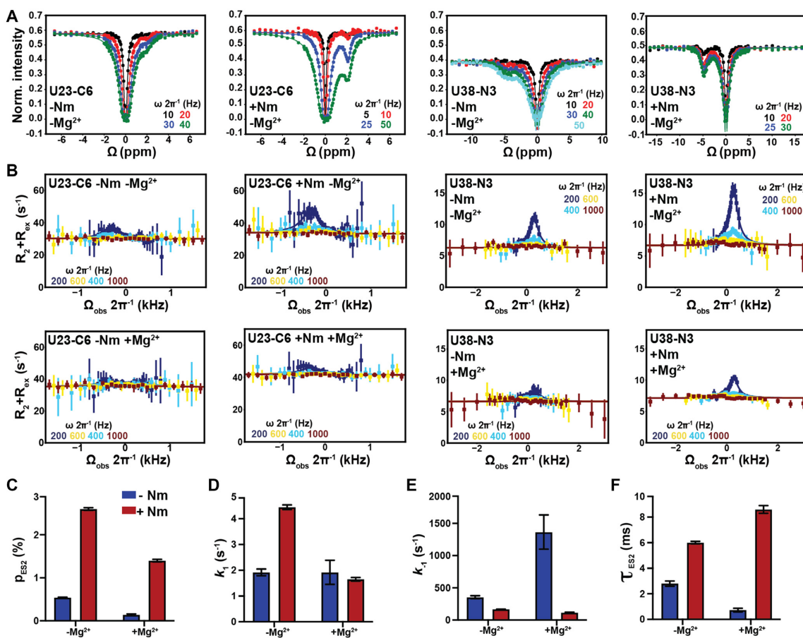
Figure 4. Impact of Nm on GS-ES2 exchange in TAR. (A) ^{13}\text{C} and ^{15}\text{N} CEST profiles in TAR and TAR-C24U25A35 in the absence of \text{Mg}^{2+} . (B) Off-resonance ^{13}\text{C} and ^{15}\text{N} R_{1\rho} RD profiles for U23-C6 and U38-N3 in TAR and TAR-C24U25A35 in the absence and presence of 1 mM of \text{Mg}^{2+} . R_{1\rho} data was fit with a two-state model using Bloch-McConnell equations. Fits of R_{1\rho} profiles were performed fixing the population to the value measured using CEST. Errors in the R_{1\rho} data were calculated as described previously (110). Spin-lock powers in CEST and R_{1\rho} are color-coded. (C-F) Comparison of p_{\text{ES2}} , k_1 and k_{-1} rate constants, and \tau_{\text{ES2}} between TAR and TAR-C24U25A35 in the absence and presence of 1 mM \text{Mg}^{2+} obtained from fitting the CEST and R_{1\rho} data. Error bars were calculated using a Monte-Carlo scheme (62).
