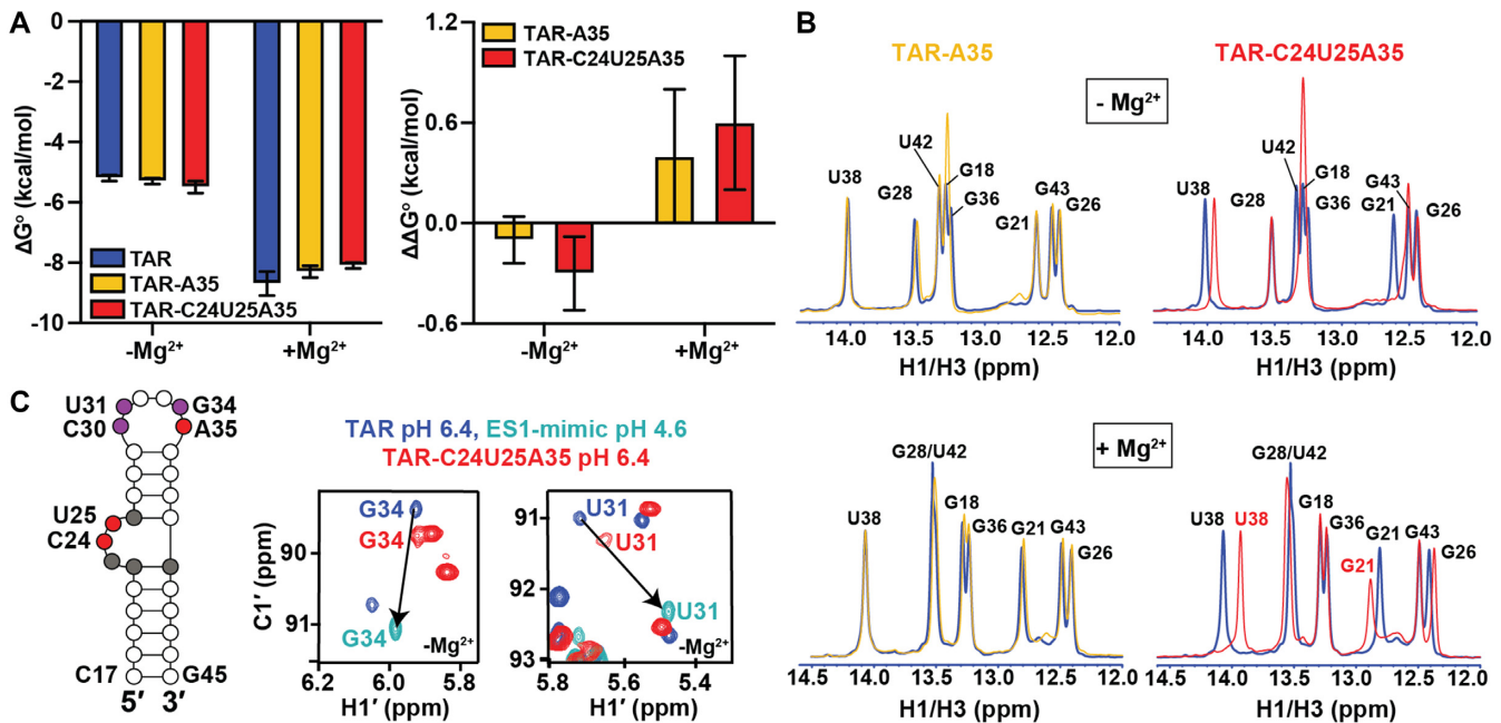
Figure 2. Impact of Nm on the thermal stability of TAR GS. (A) \Delta G^{\circ} and \Delta\Delta G^{\circ} values derived from melting curves in the absence and presence of 3 mM Mg 2+ . Error bars on \Delta G^{\circ} denote standard deviation of triplicate measurements as described in the methods. \Delta\Delta G^{\circ} = \Delta G^{\circ} (Nm - modified) - \Delta G^{\circ} (unmodified TAR). Error bars on \Delta\Delta G^{\circ} were obtained by propagating the errors from triplicate measurements (see Methods). (B) Overlays comparing 1D 1 H imino spectra for unmodified TAR (blue), TAR-A35 (yellow) and TAR-C24U25A35 (red) in the absence and presence of 3 mM Mg 2+ . All samples were unlabeled. (C) Secondary structure of TAR with Nm-modified residues shown in red, residues showing CSPs towards ES1 are in purple, and residues exhibiting CSPs due to bulge modifications are in grey. Overlay of natural abundance 2D [ 13 C, 1 H] HSQC spectra for the C1'-H1' region in TAR (pH 6.4), TAR ES1-mimic (pH 4.6) (69), and TAR-C24U25A35 (pH 6.4), in the absence of Mg 2+ . Lowering the pH to 4.6 shifts the population of TAR (structure shown in Supplementary Figure S3) to stabilize ES1 as the dominant conformation due to protonation of the A35-C30 mismatch unique to ES1 (69). Spectra with complete assignments are shown in Supplementary Figures S2 and S3.
