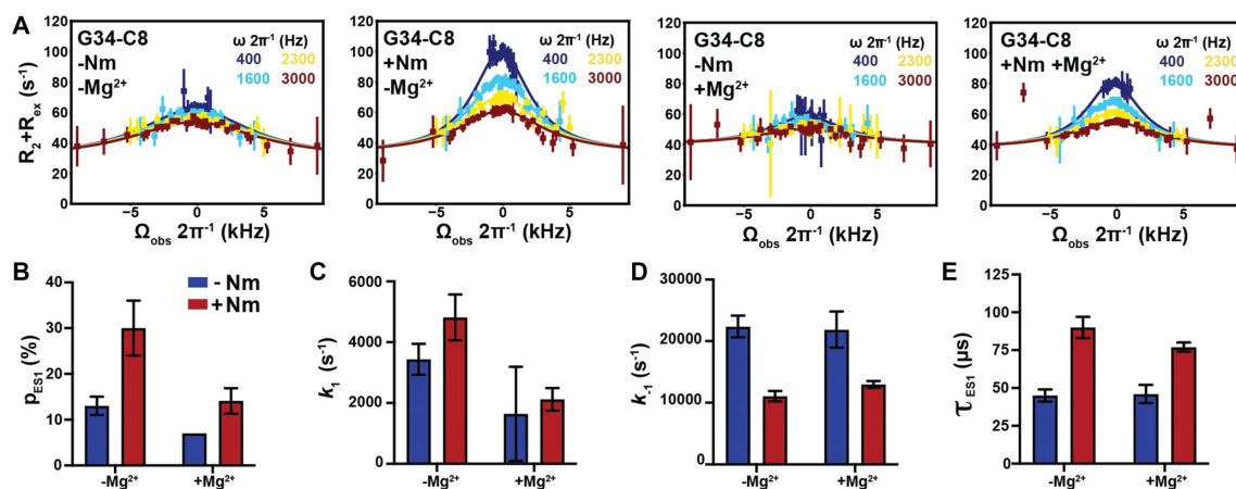
Figure 3. Impact of Nm on GS-ES1 exchange. (A) Off-resonance R_{1\rho} ^{13}\text{C} RD profiles for G34-C8 in TAR and TAR-C24U25A35 at 25°C, in the absence and presence of 1 mM \text{Mg}^{2+} . R_{1\rho} data was fit with a two-state model using Bloch-McConnell equations. Spin-lock powers are color-coded. Errors in the R_{1\rho} data were calculated as described previously (110). (B-E) Comparison of ES1 population ( p_{\text{ES1}} ), forward ( k_1 ) and backward ( k_{-1} ) rate constants, and lifetime ( \tau ) between TAR and TAR-C24U25A35, in the absence and presence of 1 mM \text{Mg}^{2+} , as obtained from fitting R_{1\rho} data. Error bars were calculated using a Monte-Carlo scheme (110).
