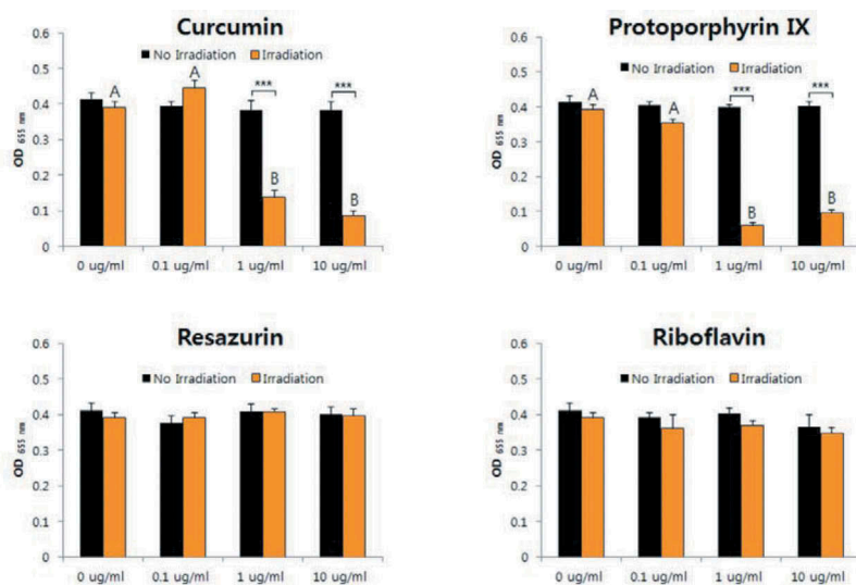
Figure 5. Photodynamic inactivation of S. mutans by four PSs. *** p < 0.001 . Different letters indicate significant differences between groups ( p < 0.05 ). Data are mean and SD values.
