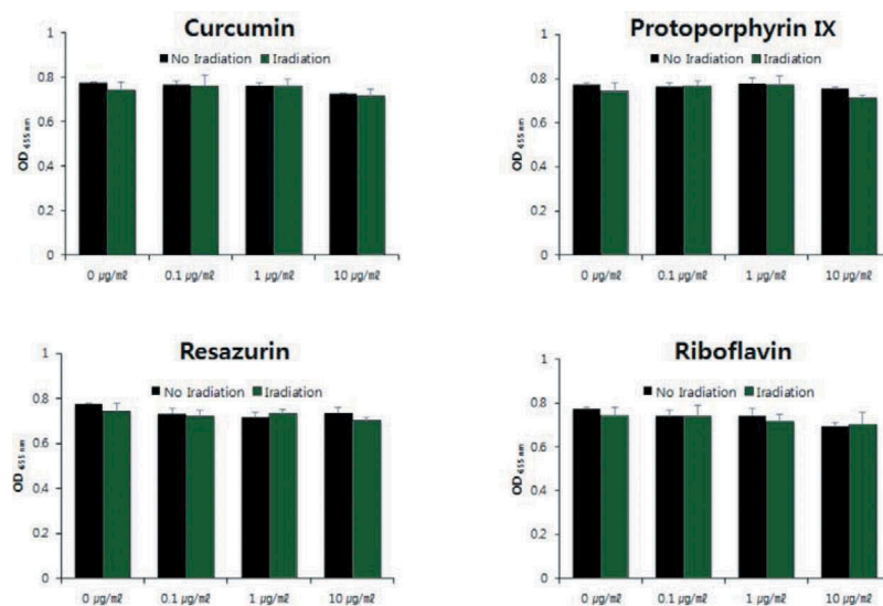
Figure 4. Photodynamic inactivation of L. gasseri by four PSs. Data are mean and SD values.
