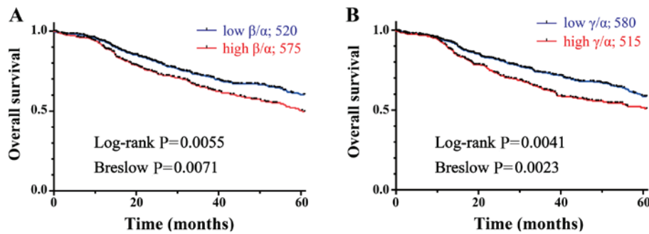
Figure 7. Survival curves of breast cancer patients based on DMTF1 isoform ratios. A breast invasive carcinoma TCGA dataset (ID: TCGA.BRCA.sampleMap/HiSeqV2) was analyzed as described in the Materials and methods. Kaplan-Meier graphs for the survival of the breast cancer patients against (A) DMTF1 \beta/\alpha and (B) DMTF1 \gamma/\alpha ratios in the corresponding groups were presented. Patient numbers were labeled behind corresponding group names. DMTF1, cyclin D binding myb-like transcription factor 1.
