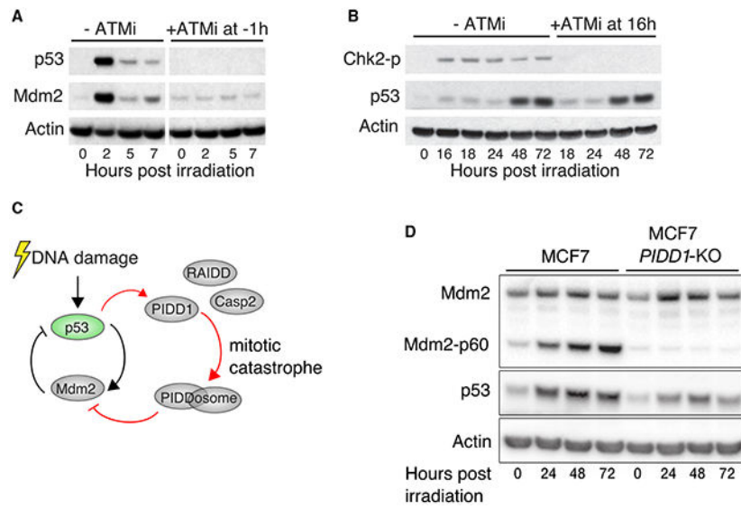
Figure 4. The Caspase-2-PIDDosome Contributes to the Switch in p53 Dynamics (original)
