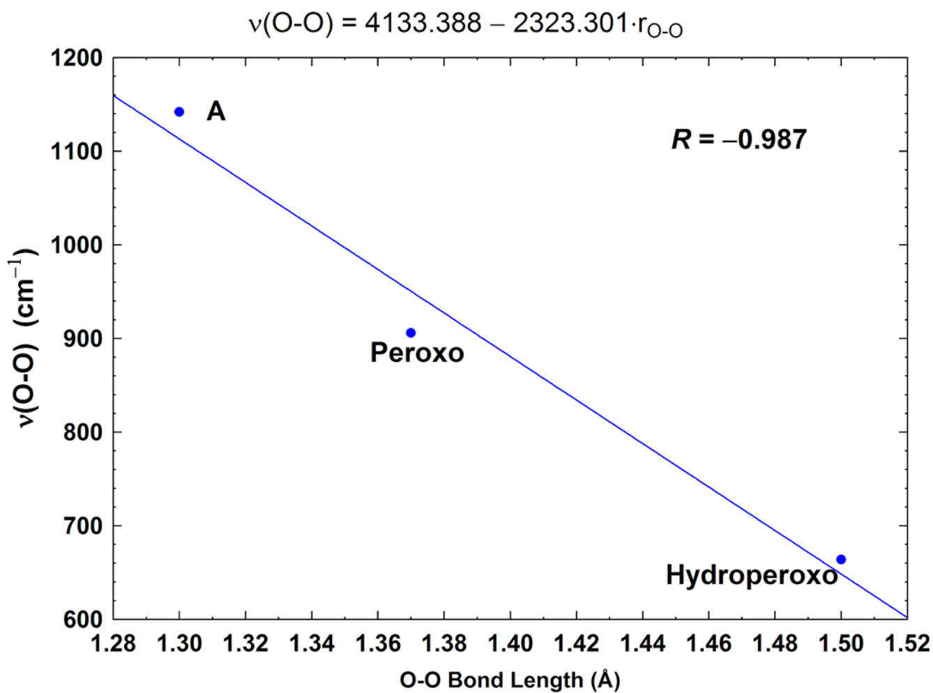
Figure 10. Correlation between the calculated O-O stretching frequencies ( \nu(\text{O-O}) , \text{cm}^{-1} ) and the O-O bond lengths ( r_{\text{O-O}} , Å). Taken with permission from Figure 6 of Ref 59, copyright © 2019 American Chemical Society.
