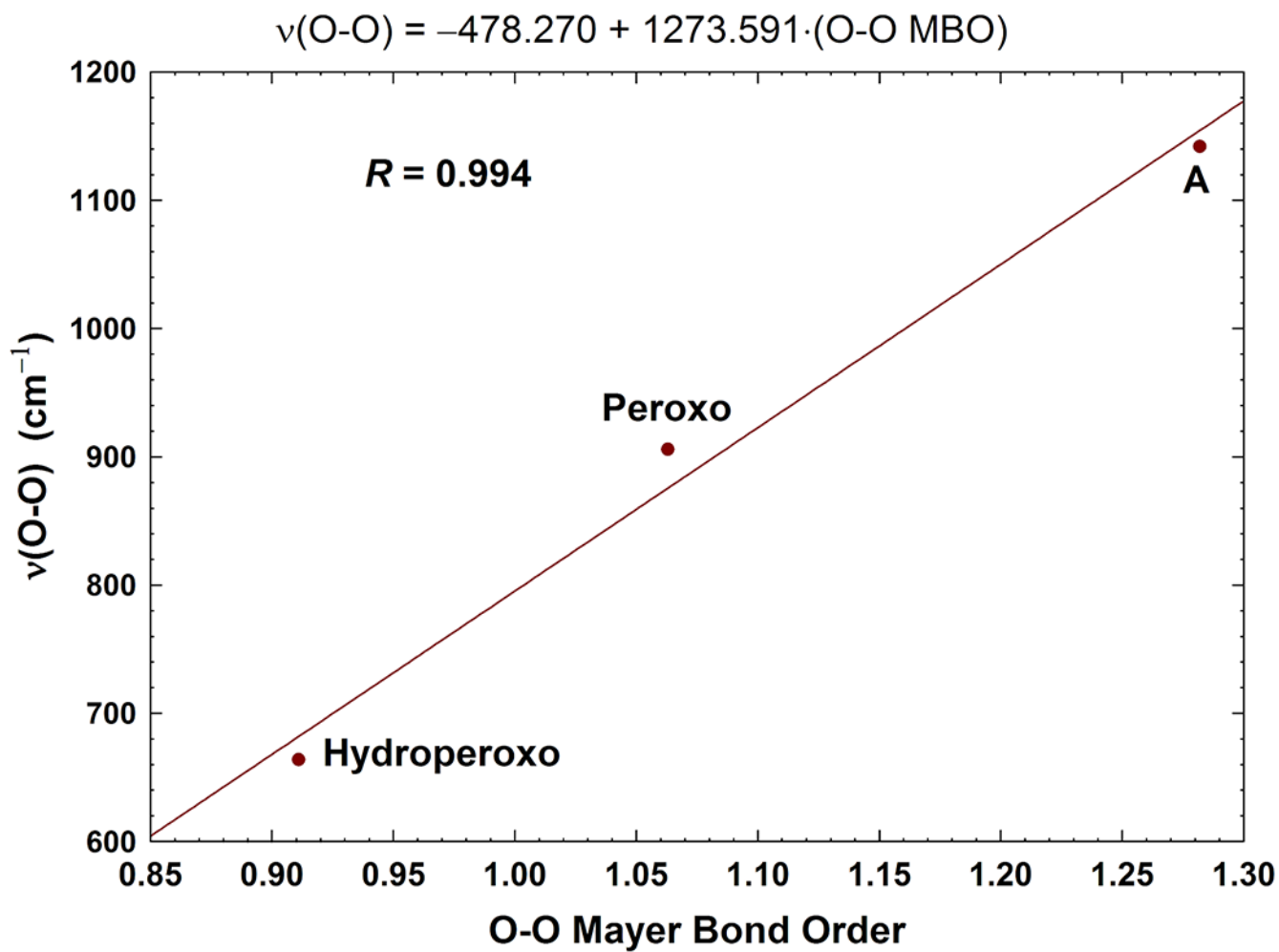
Figure 11. Correlation between the calculated O-O stretching frequencies ( \text{cm}^{-1} ) and the Mayer O-O bond orders (MBO). Taken with permission from Figure 6 of Ref 59, copyright © 2019 American Chemical Society.
