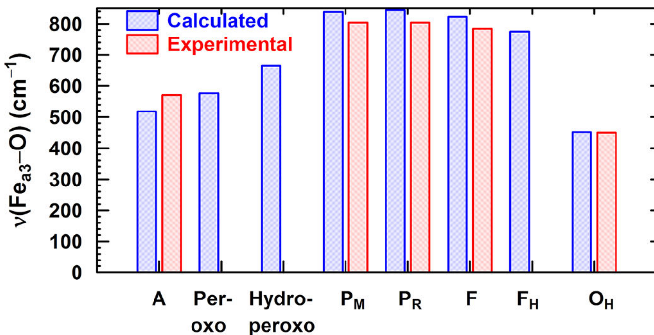
Figure 8. Calculated vs. available experimental \text{Fe}_{\text{a}3}\text{-O} vibrational stretching modes for the DNC intermediate states. Reprinted with permission from Ref 59, copyright © 2019 American Chemical Society.
