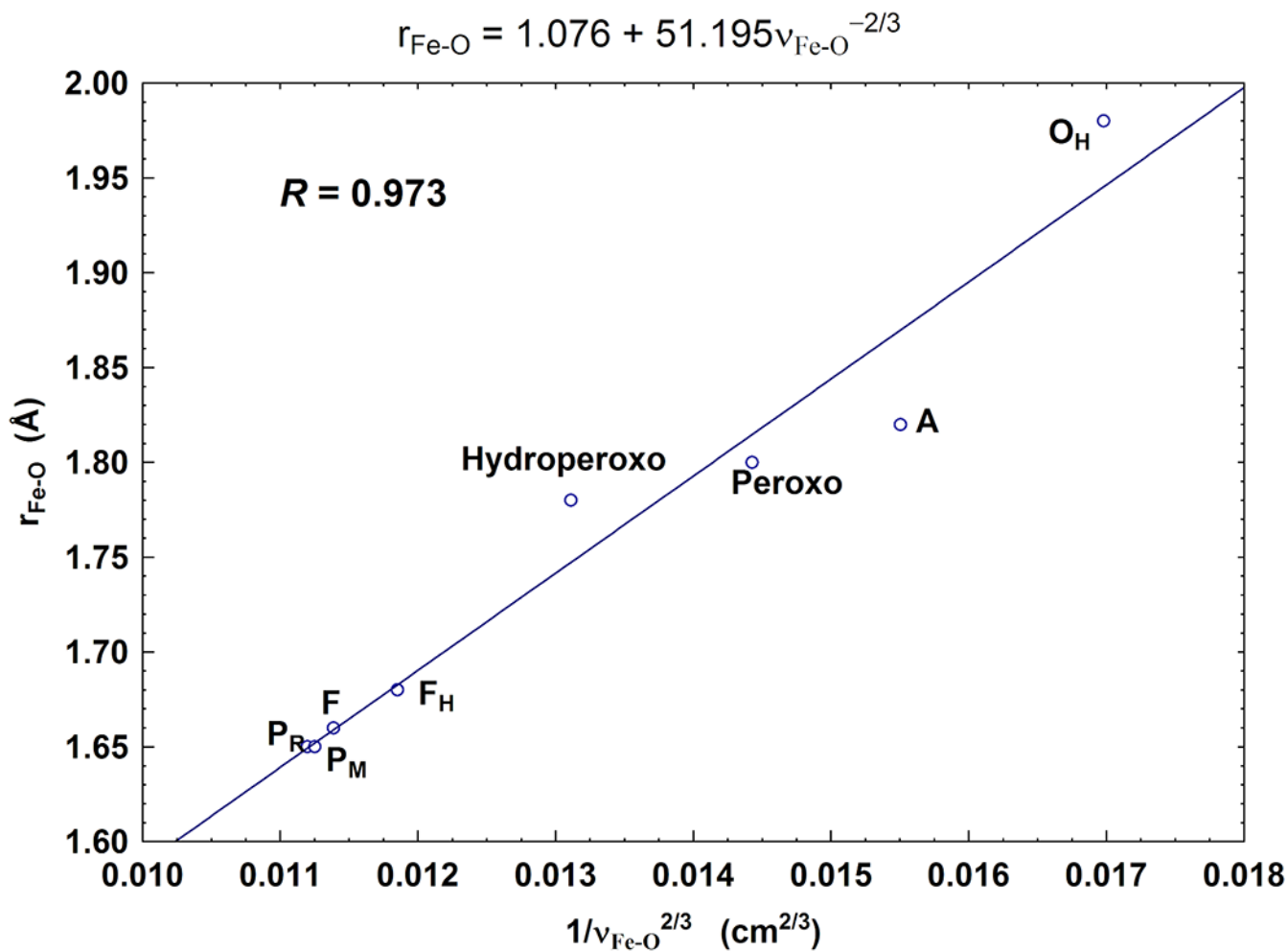
Figure 9. Correlation between the calculated \text{Fe}_{a3}\text{-O} bond lengths ( r_{\text{Fe-O}} , Å) and the corresponding \text{Fe}_{a3}\text{-O} stretch frequencies ( 1/\nu_{\text{Fe-O}}^{2/3} , based on Badger's rule) for the eight DNC state structures studied. 59 Reprint with permission from Figure 7 of Ref 59, copyright © 2019 American Chemical Society.
