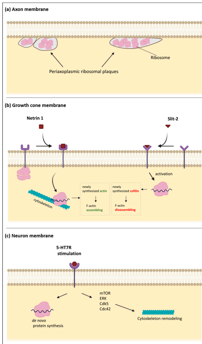
Figure 2. Schematic diagrams of the subplasmalemmal regions in specialized neuronal compartments. (a) the axonal plasma membrane is associated with “periaxoplasmic plaques”, which contain ribosomes and therefore serve as a center for intra-axonal protein synthesis. (b) The plasma membrane of the
