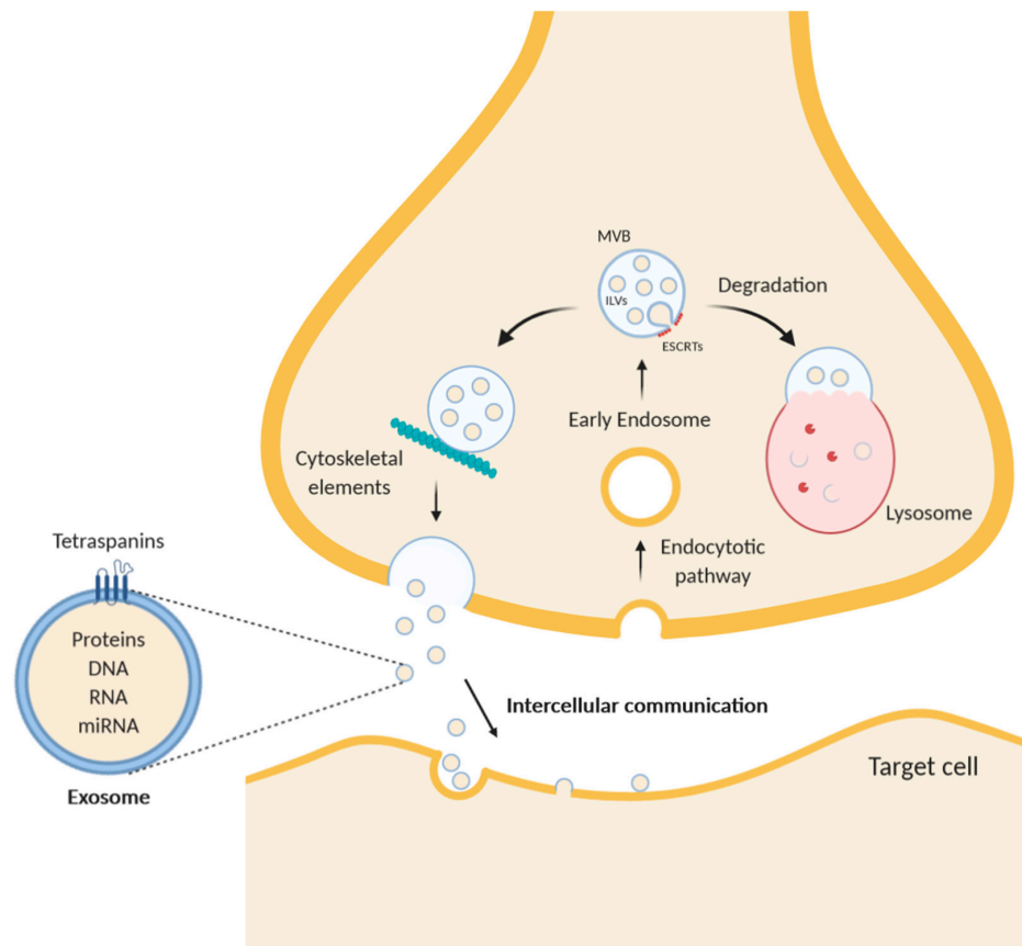
Figure 1. Schematic diagram of exosome trafficking in a neuron. While multivesicular bodies (MVBs) undergo a maturing process, the composition of the intraluminal proteins is gradually changed. The endosomal sorting complex required for transport (ESCRT) remodels the inner membrane of MVB to generate the intraluminal vesicles (ILVs), which represent exosomes inside the MVBs. After intracellular translocation mediated by cytoskeleton elements, such as F-actin, and microtubules, MVBs merge with the plasma membrane and undergo exocytosis. Alternatively, MVBs can fuse with lysosomes to degrade themselves. Exosomes contain in their lumen free proteins, RNA, microRNA, and DNA and are characterized by transmembrane proteins of the tetraspanins family.
