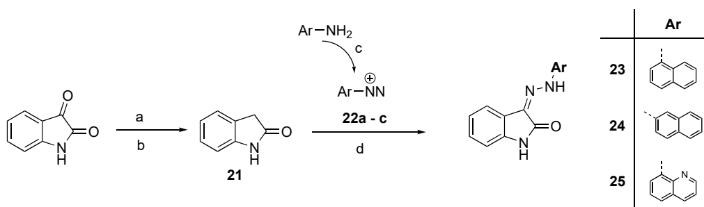
Scheme 3. Synthesis of 23–25 . Reagents and conditions: (a) \text{NH}_2\text{NH}_2 \cdot \text{H}_2\text{O} , EtOH; (b) NaOH, EtOH, \text{H}_2\text{O} , reflux; (c) \text{NaNO}_2 , \text{H}_2\text{O} , HCl 6N, 0\text{ }^\circ\text{C} ; (d) MeOH, \text{CH}_3\text{COONa} , 0\text{ }^\circ\text{C} .
