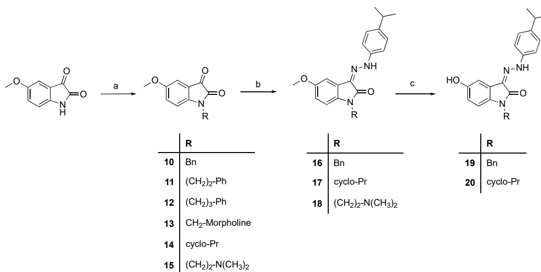
Scheme 2. Synthesis of compounds 10–20 . Reagents and conditions: (a) DMF, \text{K}_2\text{CO}_3 , 2-chloro- N,N -dimethylethylamine hydrochloride, rt, or formaldehyde, morpholine, ethanol, reflux; (b) MeOH, 4-isopropylphenylhydrazine, rt; (c) \text{BBr}_3 , \text{CH}_2\text{Cl}_2 , -70^\circ\text{C} .
