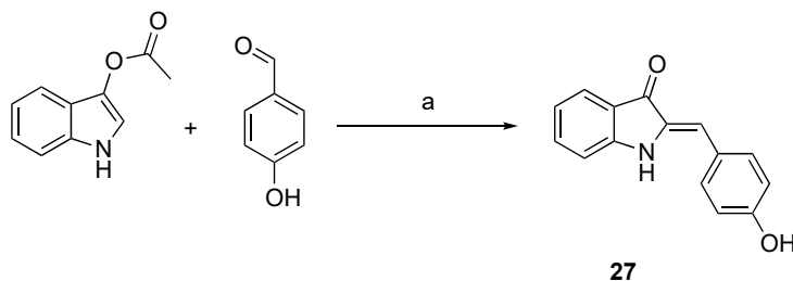
Scheme 5. Synthesis of 27 . Reagents and conditions: (a) MeOH, HCl conc., reflux, \text{N}_2 .
