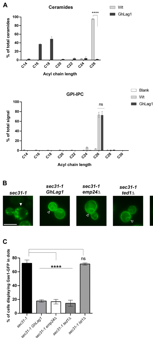
Fig. 3. ER clustering of C26 ceramide-based GPI-APs requires the presence of C26 ceramides in the membrane and interaction with the p24 complex receptor through the GPI-glycan. (A) The cellular membranes of GhLag1 mainly contain shorter C18-C16 ceramide, while the GPI anchor of Gas1-GFP still has C26 IPC as in wild-type cells. Upper graph: acyl chain length analysis by mass spectrometry (MS) of ceramides from cellular membranes of wild-type (Wt) and GhLag1p strains. Data represent the percentage of total ceramides. Mean of three independent experiments. Error bars = SD. Two-tailed, unpaired t test. **** P < 0.0001. Lower graph: acyl chain length analysis by MS of IPCs present in the GPI anchor of Gas1-GFP (GPI-IPC) expressed in wild-type and GhLag1p strains. Data represent the percentage of total IPC signals. Mean of five independent experiments. Error bars = SD. Two-tailed, unpaired t test. ns, not significant. P = 0.9134. (B) Fluorescent micrographs of sec31-1 , sec31-1 GhLag1 , sec31-1 emp24Δ , sec31-1 ted1Δ , and sec31-1 lst1Δ cells expressing galactose-inducible Gas1-GFP were incubated at 37°C for 30 min and visualized by conventional fluorescence microscopy after shifting down to 24°C. White arrowheads: ER Gas1-GFP clusters. Open arrowheads: unclustered Gas1-GFP distributed throughout the ER membrane showing the ER-characteristic nuclear ring staining. Scale bar, 5 μm. (C) Quantification of micrographs described in (B). Average percentage of the cells with dot-like Gas1-GFP structures. n ≥ 300 cells in three independent experiments. Error bars = SD. Two-tailed, unpaired t test. **** P < 0.0001.
