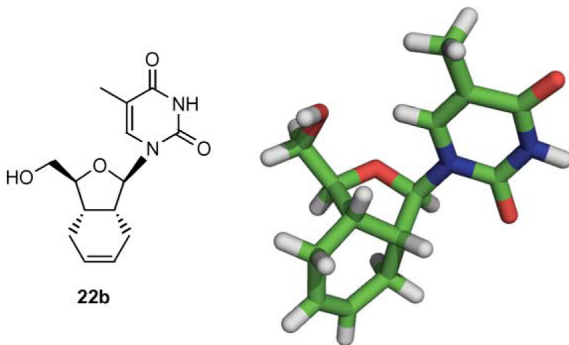
Fig. 3. Single X-ray structure of compound 22b .
