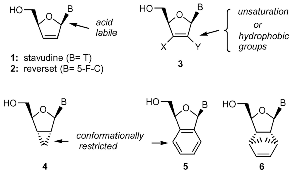
Fig. 1. Designed features of modified nucleosides.
