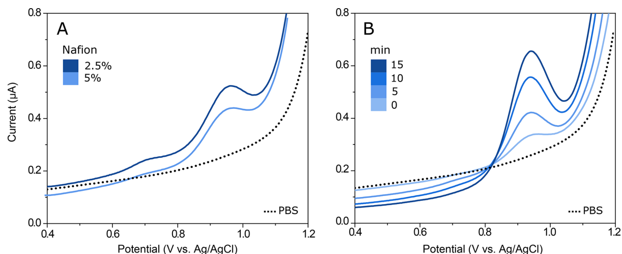
Figure 3. Characterization of the Nafion/SWCNT electrode. (A) Nafion concentration. 5 μM oxycodone with SWCNT with 2.5% Nafion and 5% Nafion. (B) Accumulation time. 5 μM oxycodone measured with SWCNT 2.5% Nafion with accumulation times 0, 5, 10, and 15 min.
