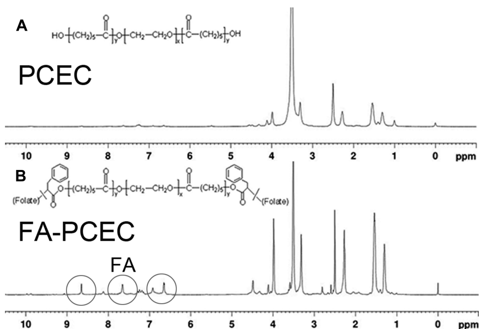
Figure 2 H-NMR spectra of PCEC (A) and FA-PCEC (B). The gray circle represents the characteristic peak of FA. Abbreviation: H-NMR, NMR hydrogen spectroscopy.
