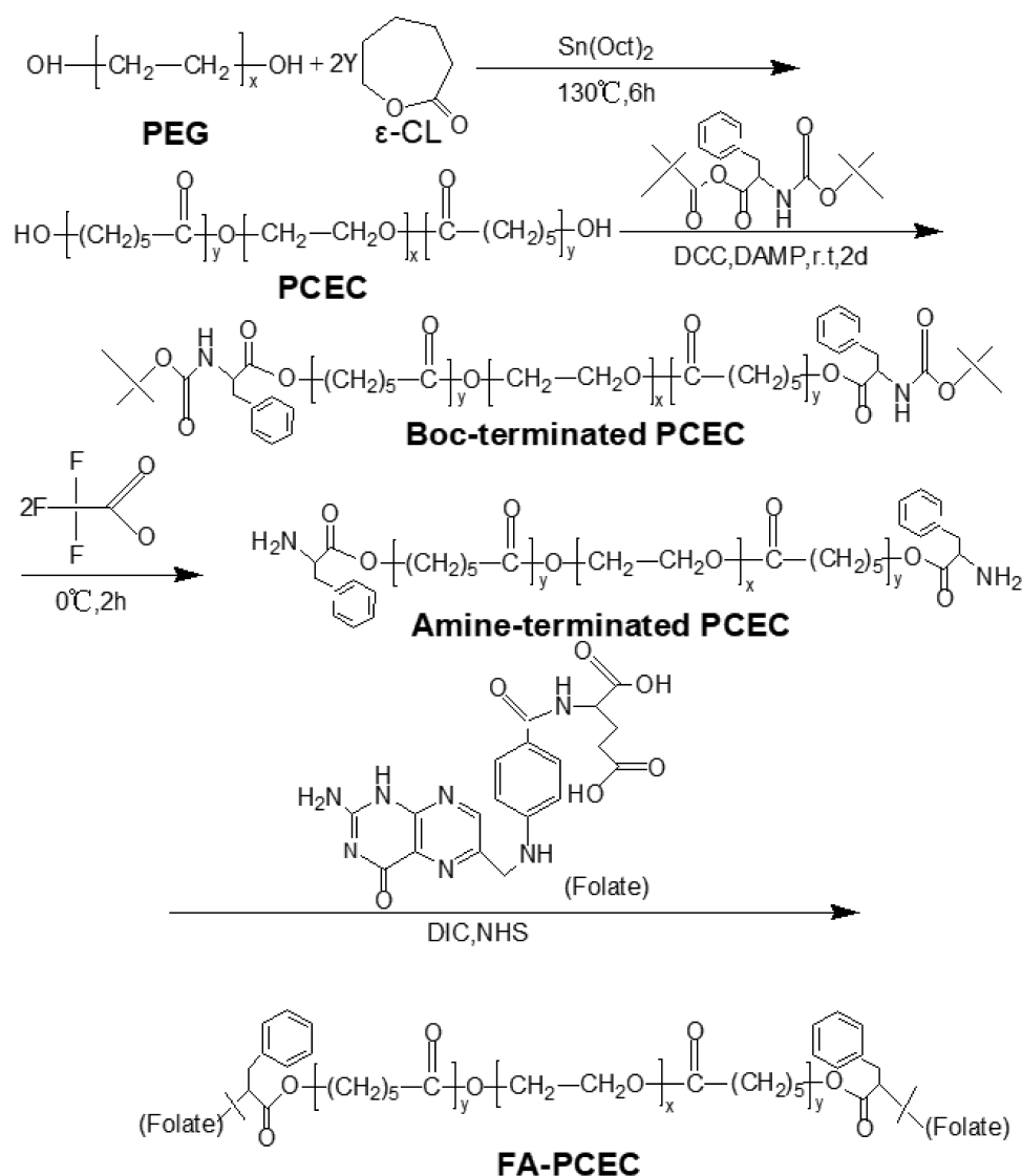
Figure 1 The synthesis route of FA-PCEC block copolymer. Abbreviation: PEG, polyethylene glycol.
