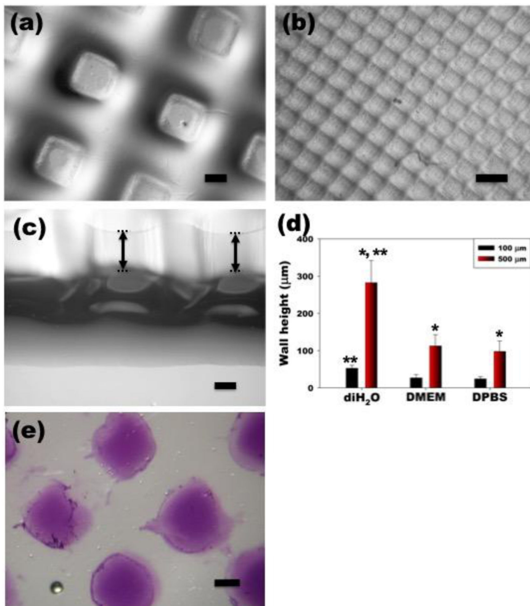
Figure 2. Optical photomicrographs and wall height measurement of dual-crosslinked OMA/PEG microwell hydrogels with various pattern sizes.
