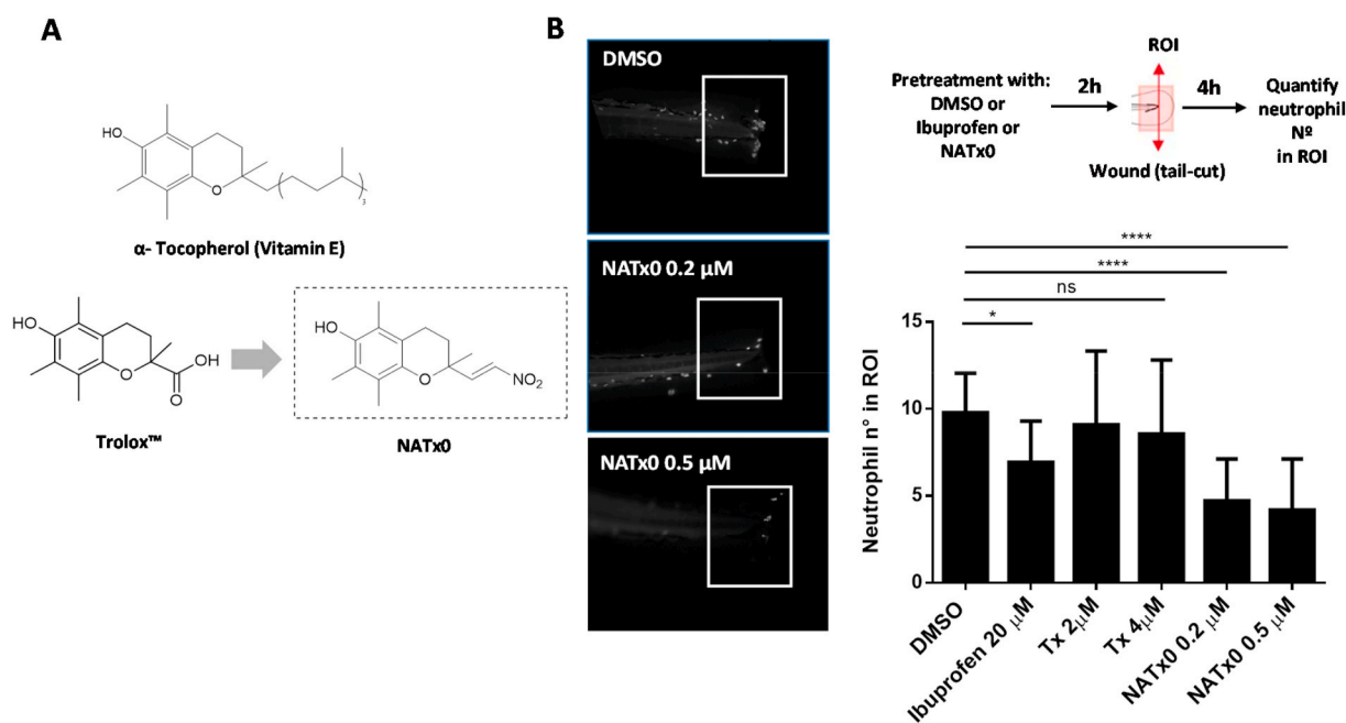
Fig. 1. NATx0 inhibits acute inflammatory response in zebrafish larvae. A , \alpha -Tocopherol Vitamin E, its hydrosoluble form (Trolox TM ) and Trolox-derived nitroalkene NATx0 chemical structures are shown. B , NATx0 inhibits neutrophil recruitment in an acute inflammatory assay in zebrafish larvae. Briefly, 3 dpf zebrafish neutrophil-specific larvae Tg (mpx:GFP) were pretreated with NATx0, Trolox or Ibuprofen for 2 h and wounded in tail fins by transection with a scalpel. After, larvae were incubated again in the presence of the compounds during 4 h and then recruited neutrophils were imaged and quantified. Experimental diagram and representative pictures obtained corresponding to DMSO, NATx0 0.2 \mu M and NATx0 0.5 \mu M are shown. Graph represent the quantification of the neutrophils recruited to wounded fins inside a defined ROI. Bar graphs shown are the mean \pm S.D. (error bars) of at least 17 larvae in each condition. Data represents two independent experiments. Statistical analysis: One-way ANOVA with Bonferroni's multiple comparison test, * = 0.0487; DMSO vs Tx 2 \mu M ns = 0.992; DMSO vs Tx 4 \mu M ns = 0.844; **** < 0.0001; **** < 0.0001.
