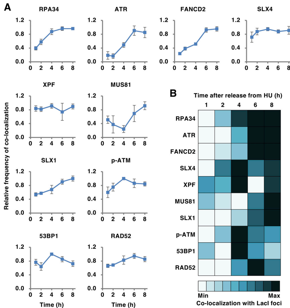
Figure 2. DDR factors associated with ATR, FA, and ATM pathways accumulate at the LacI-bound lacO array with distinct dynamics. (A) U2OS 40–2–6 ER-LacI cells were synchronized with 2.5 mM HU for 18 h and released into fresh medium containing 1 \mu M 4-OH-tamoxifen for the indicated times. Cells were then double immunostained with anti-LacI antibody and the indicated antibodies, followed by DAPI staining and analysis. Colocalization frequencies of the indicated foci with the LacI foci are shown, with maximum value of the colocalization frequency for each factor set at 1. Values depicted are means \pm SD from three independent experiments. (B) The spatiotemporal heatmap depicts the accumulation kinetics of the DDR factors. The maximum–minimum range of the relative frequency of colocalization shown in (A) was calculated for each factor, then each range was equally divided into 10 fractions, which were assigned colors as indicated in the bottom panel.
