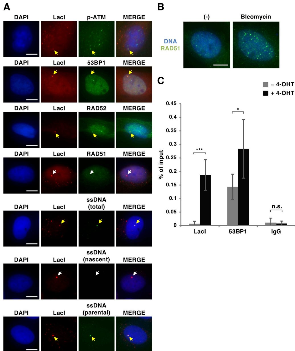
Figure S2. Recruitment of various DDR proteins to lacO arrays in U2OS 40–2–6 ER-Lacl cells. (A) U2OS 40–2–6 ER-Lacl cells treated with 1 \mu M 4-OHT for 2 h were double immunostained with the indicated antibodies and counterstained with DAPI. ssDNA was stained with anti-BrdU antibody under non-denaturing conditions. For detection of total ssDNA, DNA was labeled for 24 h with 10 \mu M BrdU. For detection of nascent-strand ssDNA, newly synthesized DNA was labeled with BrdU during treatment with 4-OHT. For detection of parental-strand ssDNA, DNA was labeled with 10 \mu M BrdU for 20 h, followed by a chase in fresh medium without BrdU for 2 h before addition of 4-OHT. Representative images are shown, and the colocalization frequencies are shown in Fig. 1 D. Yellow arrows indicate colocalization of DDR proteins with the foci of HA-Lacl, and white arrows indicate noncolocalization. Scale bars, 10 \mu m. (B) The antibody used in this study can detect bleomycin-induced RAD51 foci. U2OS 40–2–6 ER-Lacl cells were treated with 8 \mu M Bleomycin for 18 h, then immunostained with anti-RAD51 antibody, followed by DAPI staining. Representative images are shown. Scale bar, 10 \mu m. (C) U2OS 40–2–6 ER-Lacl cells treated with 1 \mu M 4-OHT or a control vehicle (EtOH) for 2 h were subjected to ChIP-quantitative PCR analysis using the indicated antibodies. Enrichment of the lacO sequences is shown as the percent of input DNA. Means \pm SD are shown ( n = 6 for control rabbit IgG; n = 7 for Lacl and 53BP1). *, P < 0.05 ; ***, P < 0.001 ; n.s., not significant (two-tailed Student's t test).
