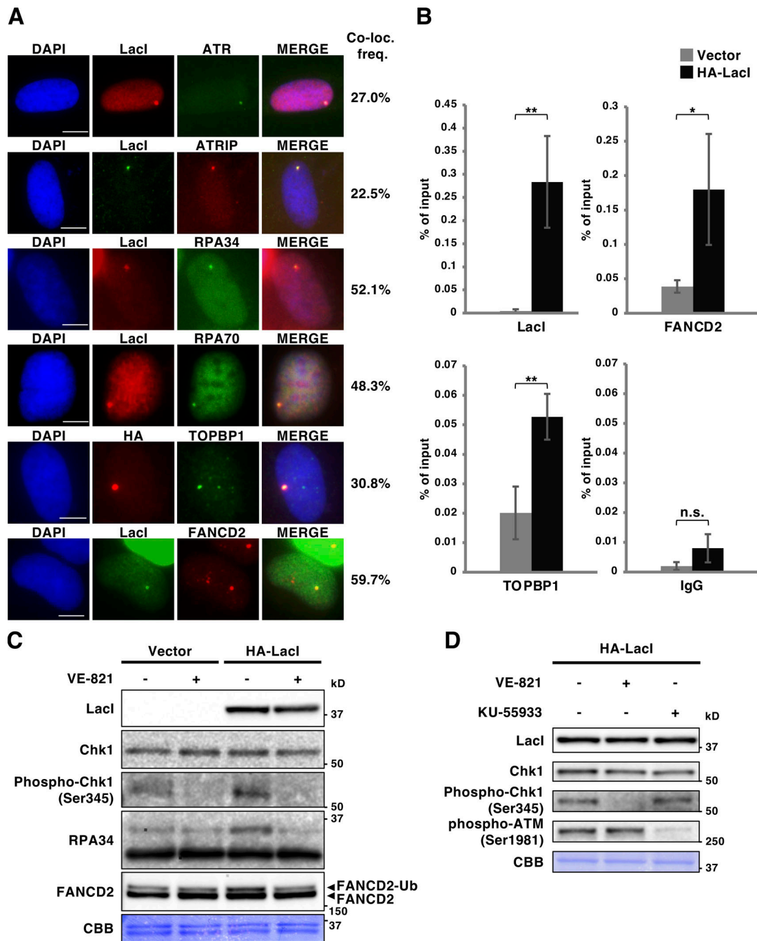
Figure S1. Recruitment of various DDR proteins to lacO arrays after transient expression of HA-Lacl in U2OS 2-6-3 cells. (A) U2OS 2-6-3 cells were transfected with HA-Lacl expression vector for 24 h using Lipofectamine 2000 reagent (Invitrogen) and then double immunostained with the indicated antibodies, followed by DAPI staining. Representative images and colocalization frequencies (%) of DDR-protein foci with Lacl foci are shown. Values were calculated from the sum scores of at least two independent experiments. Scale bars, 10 \mu m. (B) U2OS 2-6-3 cells were transfected with the empty or the HA-Lacl expression vectors for 24 h and then subjected to ChIP-quantitative PCR analysis with the indicated antibodies. Quantitative PCR was performed with primer pairs to detect lacO sequences. Results are shown as the percentage of input DNA. Means \pm SD are shown ( n = 4 ). *, P < 0.05 ; **, P < 0.01 ; n.s., not significant (two-tailed Student's t test). (C and D) U2OS 2-6-3 cells transfected as in (B) were treated with 10 \mu M VE-821 (ATR/ATM inhibitor), 10 \mu M KU-55933 (ATM inhibitor), or a control vehicle (DMSO) for 6 h and then subjected to immunoblotting. Data are representative of two or more independent experiments. In this experimental condition, VE-821 selectively inhibited ATR-mediated phosphorylation of Chk1 (Ser345), but not autophosphorylation of ATM (Ser1981). CBB, Coomassie Brilliant Blue; FANCD2-Ub, monoubiquitinated FANCD2.
