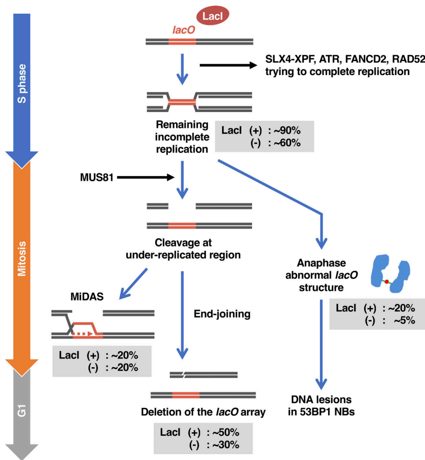
Figure 8. A model of the fate of underreplicated DNA regions in the lacO array. Even in the absence of LacI binding, the lacO array is a difficult-to-replicate region, like other repeat sequences, and contains underreplicated lesions (~60% on the basis of the data shown in Fig. 4 C), which persist until late G2/M phase. Replication stress by LacI binding to the array further increases the frequency of cells with underreplicated DNA lesions (~90%). To try to complete replication of the array during S phase, cells activate the DDR, in which one-ended DSB is first generated by SLX4–XPF-mediated DNA cleavage. Excess ssDNA is then generated by unidentified exonucleases, which in turn recruit ATR, FANCD2, and RAD52. ATR and FANCD2 are interdependently recruited. The DDR may promote completion of replication, because SLX4 and ATR inhibition exacerbates mitotic abnormality induced by LacI. The underreplicated intermediates persisting until late G2/M phase are processed by MUS81-mediated cleavage in early mitosis. Note that cleaved strands are arbitrary in the figure, because it remains unclear whether the cleavage occurs in the leading or lagging strand templates. Cleavage at lacO can promote MiDAS (~20% in the absence or presence of LacI; Fig. 4 G) or end joining that results in deletion of the loci (~30% in the absence of LacI and ~50% in the presence of LacI; Fig. 5 B). A fraction of the lacO arrays escape from the cleavage and remain underreplicated until anaphase, leading to the anaphase abnormal lacO structure (~5% in the absence of LacI and ~20% in the presence of LacI; Fig. 6 B) and the formation of 53BP1 NBs in daughter G1 cells (~5% in the absence of LacI and ~20% in the presence of LacI; Fig. 6 E).
