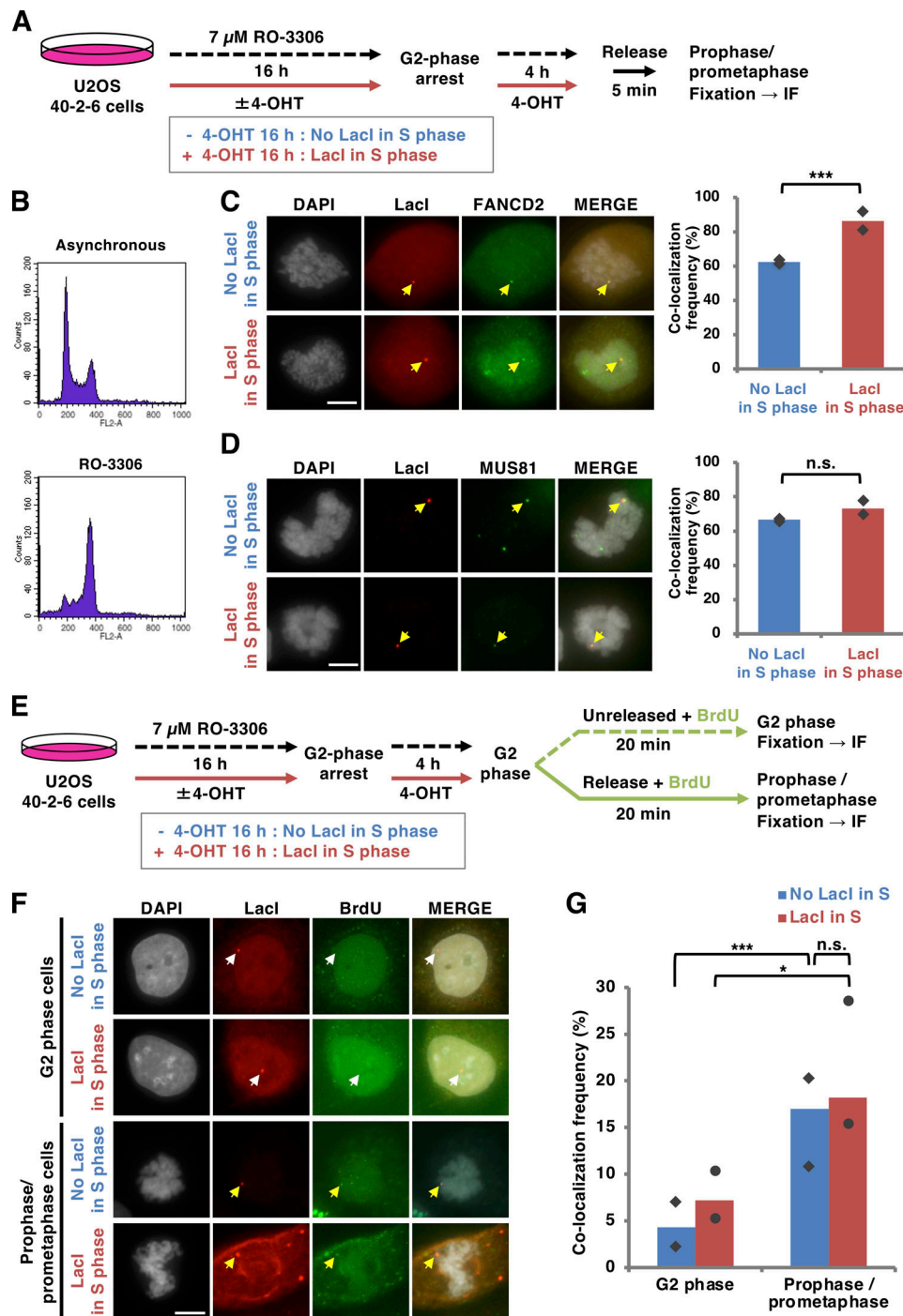
Figure 4. FANCD2 and MUS81 accumulate on the lacO array in mitosis, where MiDAS is activated, and Lacl binding during S phase increases FANCD2 colocalization with lacO . (A) Experimental scheme. U2OS 40–2–6 ER-Lacl cells were synchronized in late G2 phase with 7 \mu M RO-3306 treatment for 20 h and 1 \mu M 4-OHT for 20 h or the last 4 h. G2-arrested cells were then released into fresh medium for 5 min and subjected to double immunostaining, DAPI staining, and analysis. (B) Confirmation of G2-phase synchronization with RO-3306. U2OS 40–2–6 ER-Lacl cells synchronized in G2 phase by incubation with 7 \mu M RO-3306 for 16 h were subjected to FACS analysis. (C and D) Representative images (left) and colocalization frequencies (right) are shown. Values were calculated from the sum scores of two independent experiments. ***, P < 0.001 ; n.s., not significant ( \chi^2 test). Individual data points from the two independent experiments are also shown. Yellow arrows indicate colocalization of FANCD2 (C) or MUS81 (D) with the Lacl foci. Scale bars, 10 \mu m. (E) Experimental workflow for MiDAS detection. U2OS 40–2–6 ER-Lacl cells were synchronized in late G2 phase as described in A. The G2-arrested cells were released or left unreleased, in each case for 20 min in the presence of 10 \mu M BrdU. DNA was denatured by treatment with HCl for detection of DNA labeled with BrdU. Cells were then double immunostained with anti-Lacl and anti-BrdU antibodies, followed by DAPI staining and analysis. (F) Representative images of G2-arrested cells or prophase/prometaphase cells with Lacl foci. BrdU incorporation (indicating MiDAS) was detected specifically in mitotic cells (yellow arrows), but not in G2 cells (white arrows). Scale bar, 10 \mu m. (G) The graph indicates colocalization frequencies of BrdU foci with Lacl foci in G2 phase and prophase/prometaphase cells. Values were calculated from the sum scores of two independent experiments. *, P < 0.05 ; ***, P < 0.001 ; n.s., not significant ( \chi^2 test). Individual data points from the two independent experiments are also shown.
